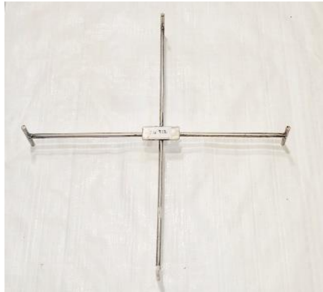
FIG. 2 (c) TEMPLATE TO MEASURE EXPANDED DIMENSIONS
