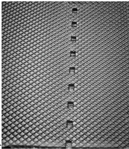
FIG. 5 (a) ULTRASONIC SEAM WELD
