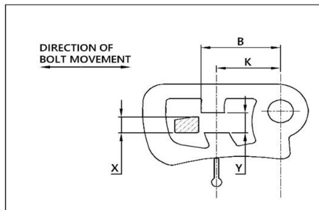
FIG. 1 LEVER GATE AND KEYHOLE ARE NEARLY ALIGNED ( R \leq 1.5 )
