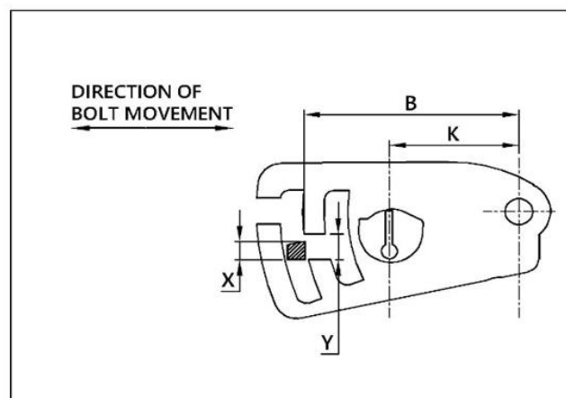
FIG. 2 LEVER GATE AWAY FROM KEYHOLE ( R > 1.5 )
