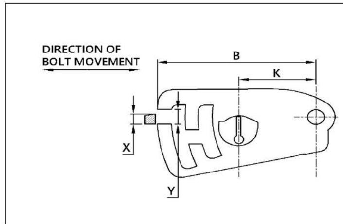
FIG. 3 LEVER GATE FURTHER AWAY FROM KEYHOLE ( R \gg 1.5 )
