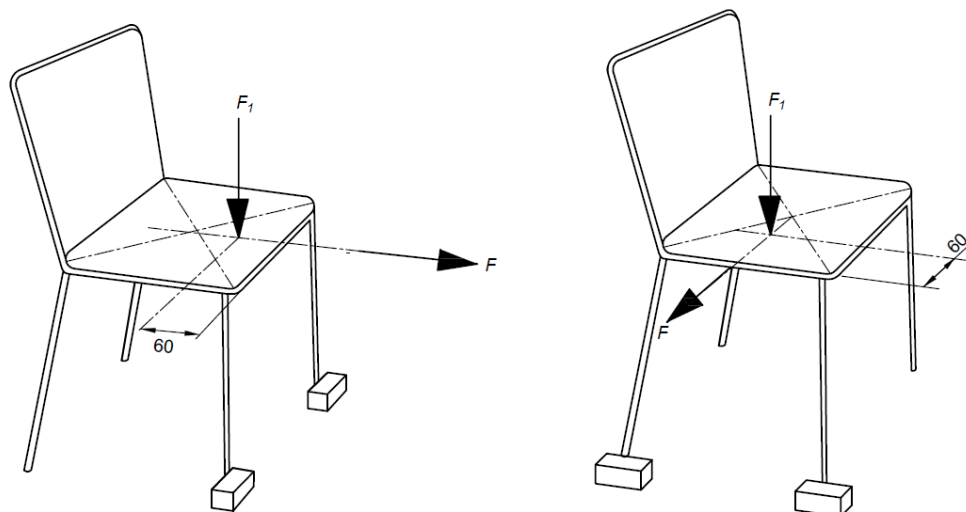
FIG. 1 FORWARDS OVERBALANCING AND SIDEWAYS OVERBALANCING FOR CHAIRS WITHOUT ARMS
