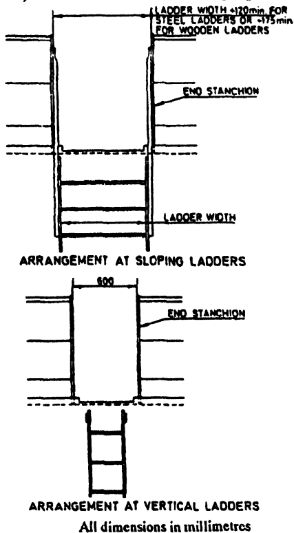
FIG. 7 TYPICAL ARRANGEMENTS OF GUARDRAILS AT LADDERS
