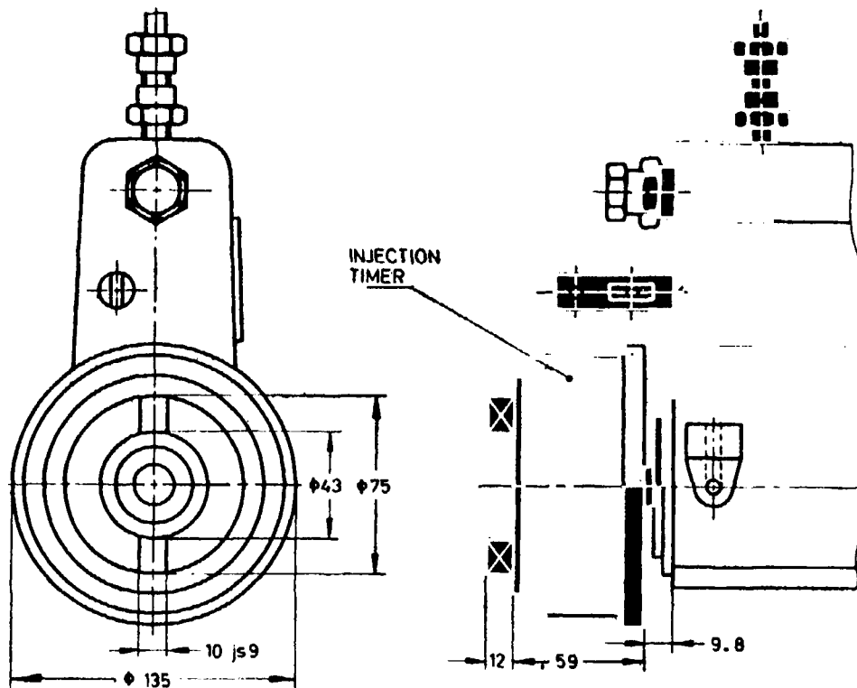
FIG. 5 ASSEMBLY OF THE F. I. PUMP WITH A TYPICAL INJECTION TIMER
