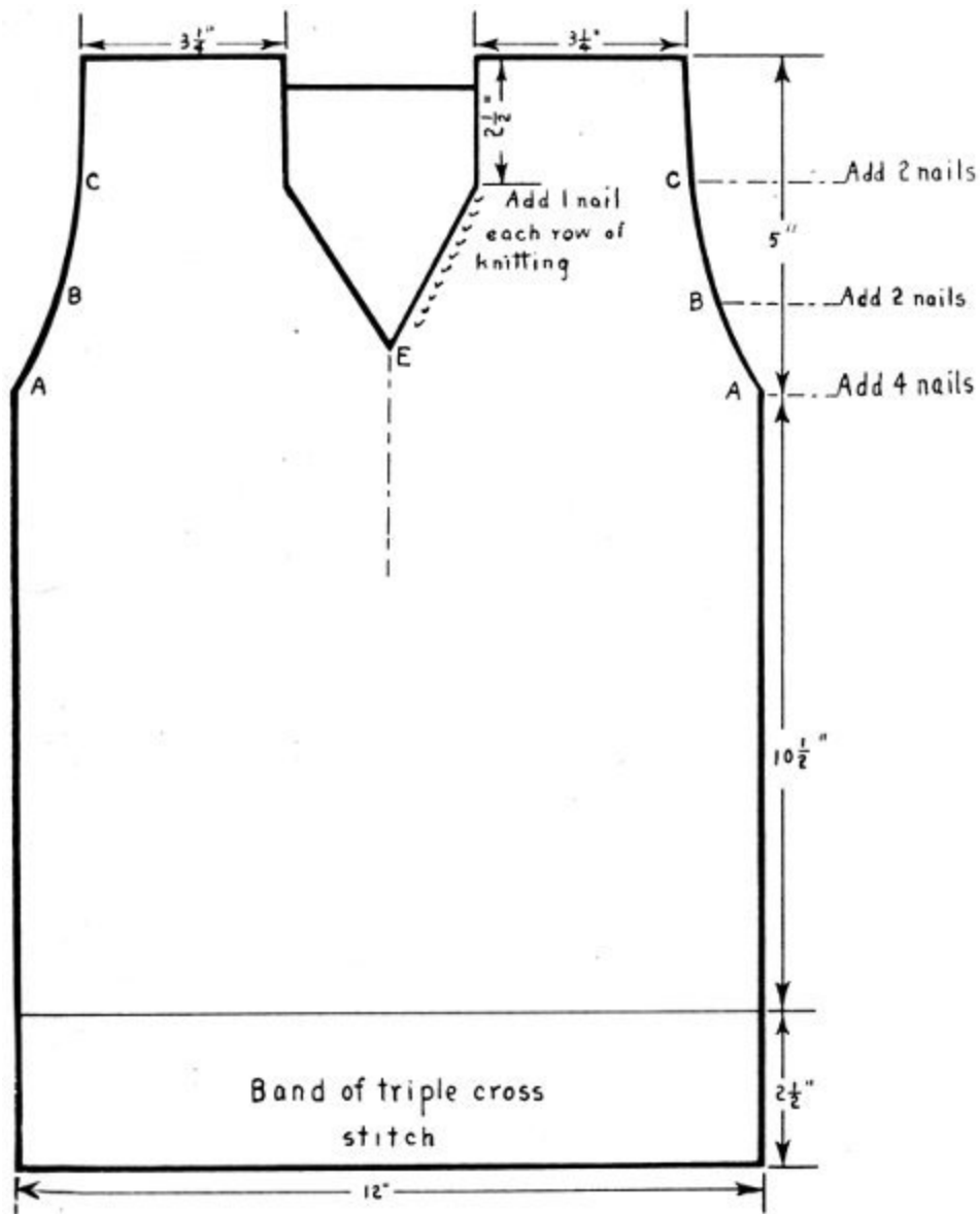
Fig. 40. Pattern for Front of Boy's Slipover Sweater.
