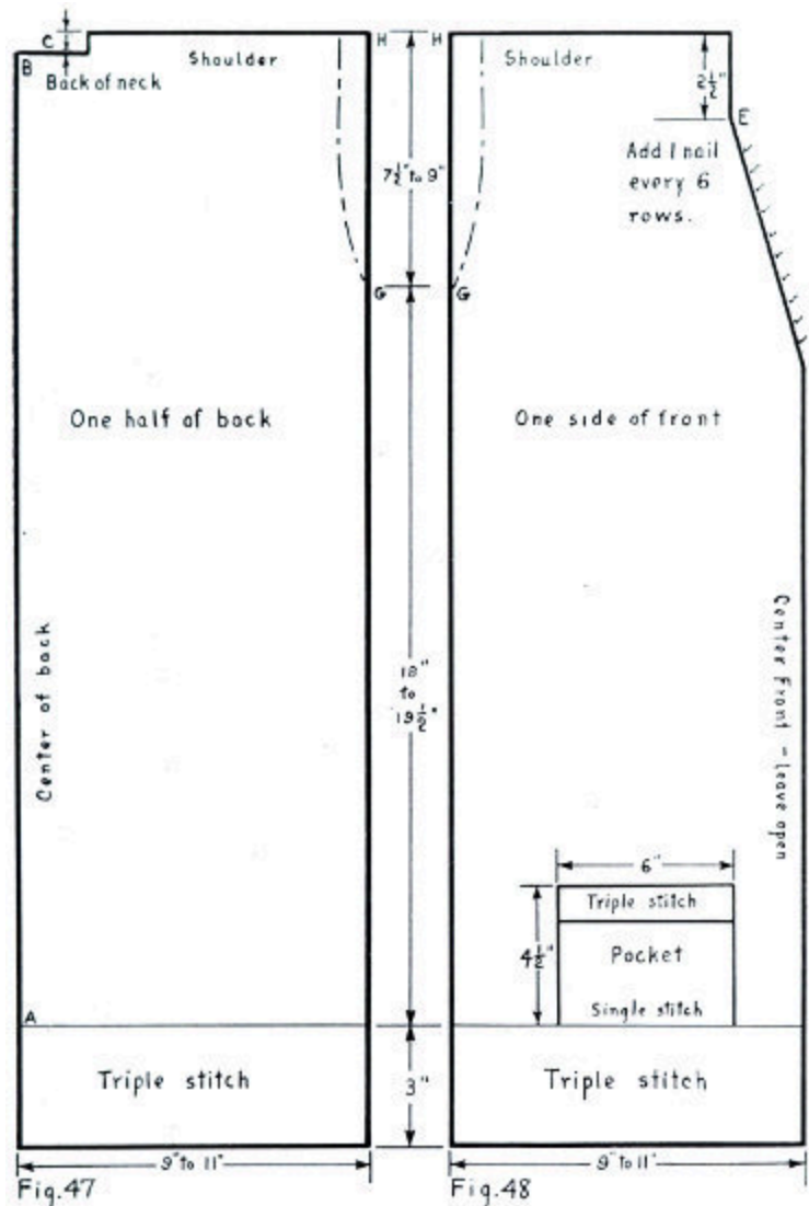
MAN'S SWEATER (Front and back)
