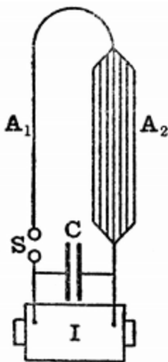
FIG. 13.—SLABY'S LOOP RADIATOR.
