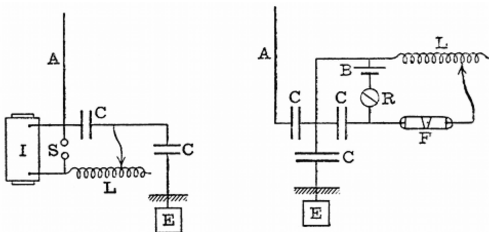
FIG. 25.—LODGE-MUIRHEAD SYNTONIC RECEIVER.
