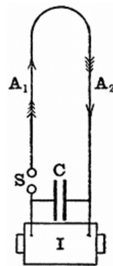
FIG. 12.—NON-RADIATIVE CLOSED LOOP AERIAL.
