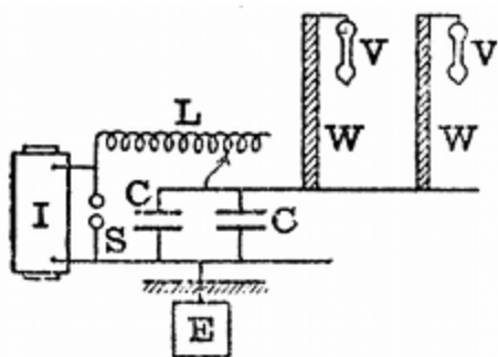
FIG. 22.—SEIBT'S APPARATUS FOR EXHIBITING ELECTRIC RESONANCE. I, induction coil; S, spark gap; CC, condensers; L, variable inductance; E, earth plate; WW, wire spirals; VV, vacuum tubes.
