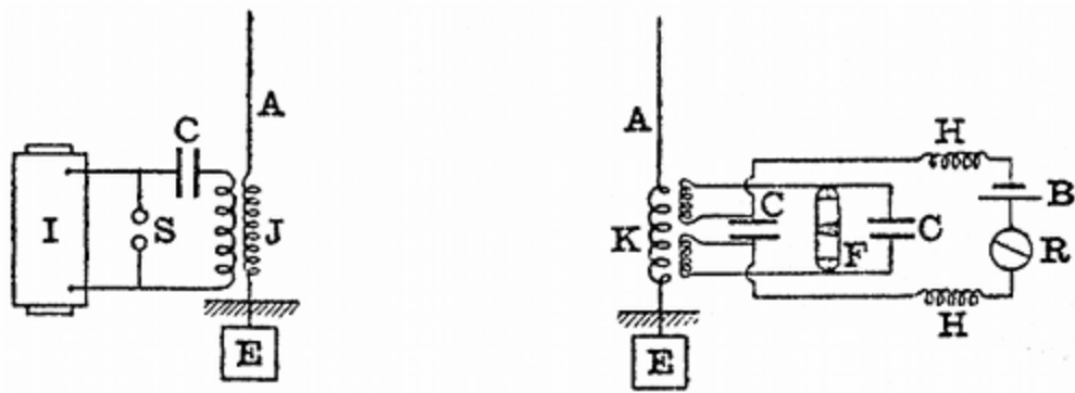
FIG. 23.—MARCONI TRANSMITTER AND RECEIVER.
