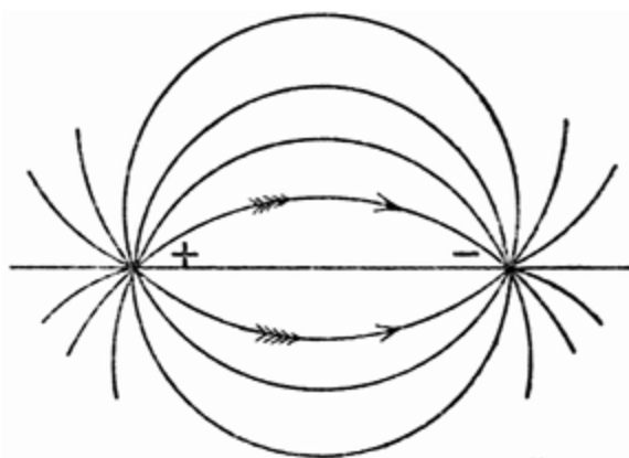
FIG. 1.—LINES OF ELECTRIC STRAIN BETWEEN A POSITIVE AND NEGATIVE ELECTRON AT REST.
