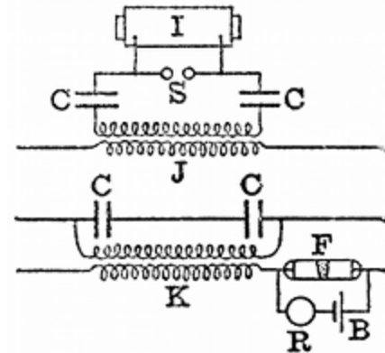
FIG. 21.—BRAUN'S NON-EARTHED RECEIVER. I, induction coil; CC, condensers; S, spark gap; J, transmitting jig; K, receiving jig; F, filings tube; R, relay; B, battery.
