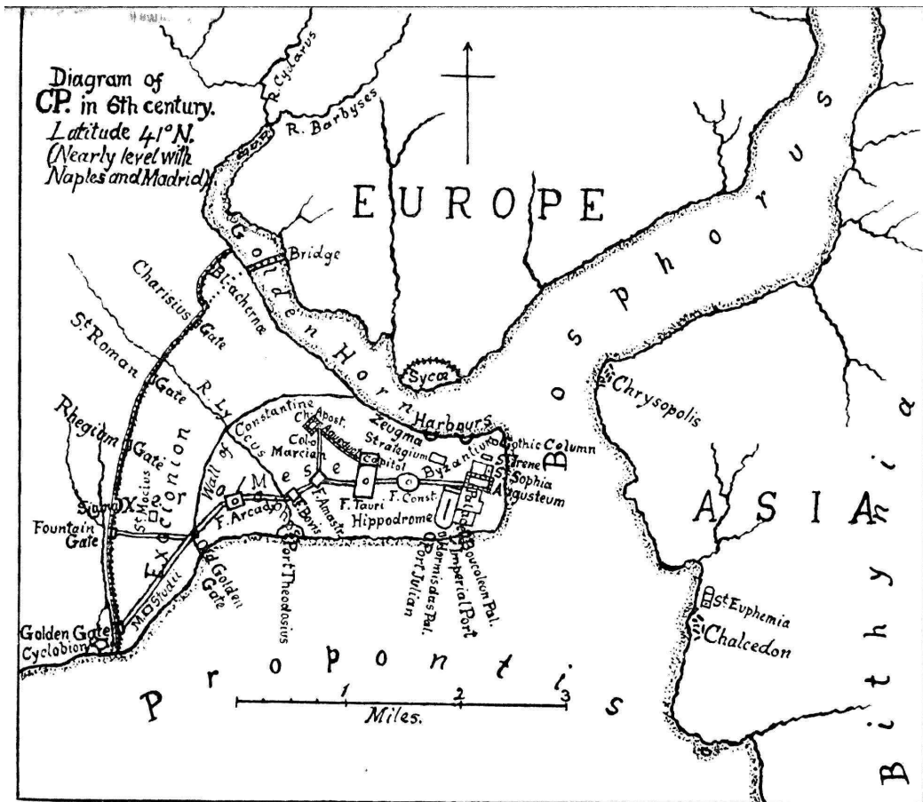
Diagram of CP. in 6th century. Latitude 41° N. (Nearly level with Naples and Madrid)
