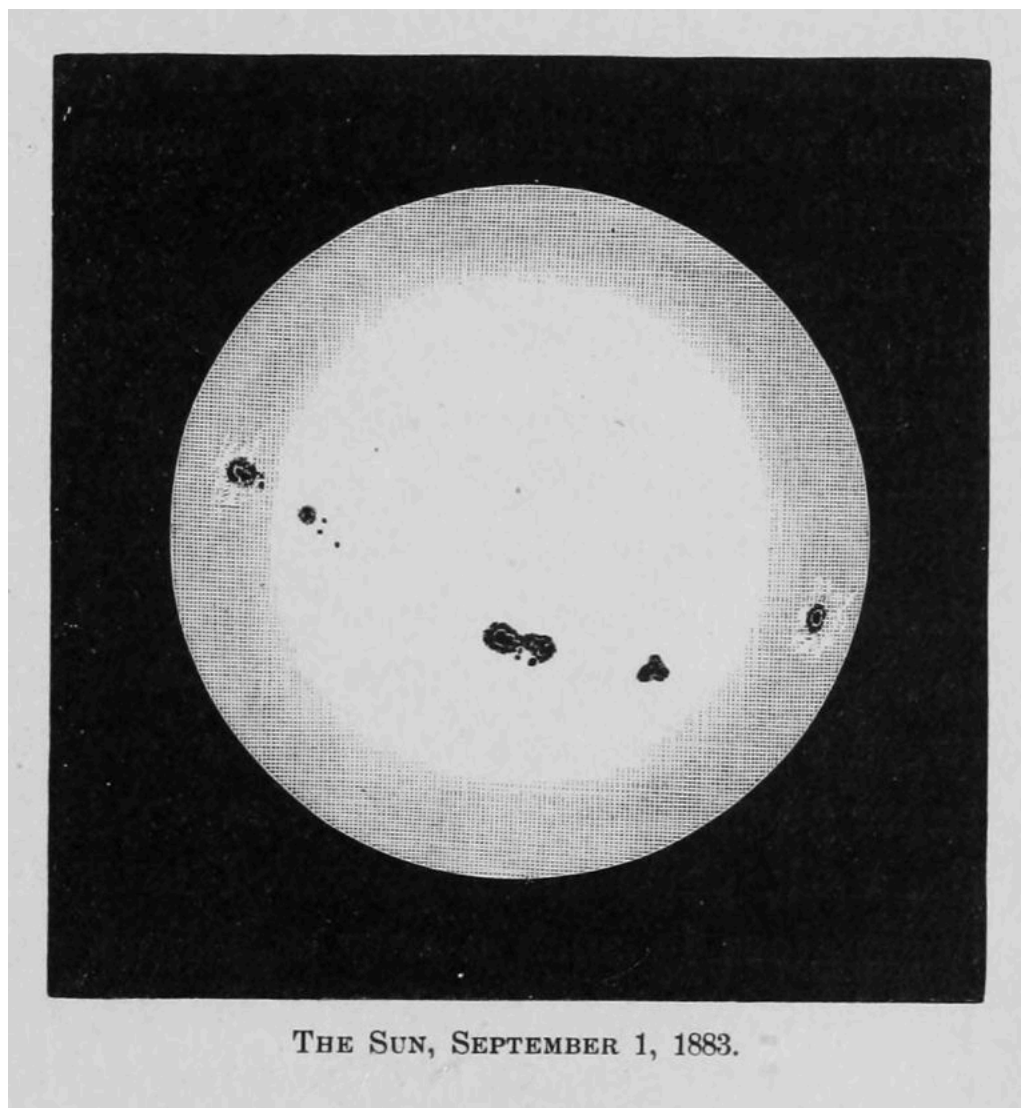
THE SUN, SEPTEMBER 1, 1883.
