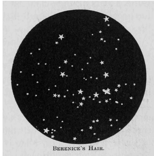
BERENICE'S HAIR.
