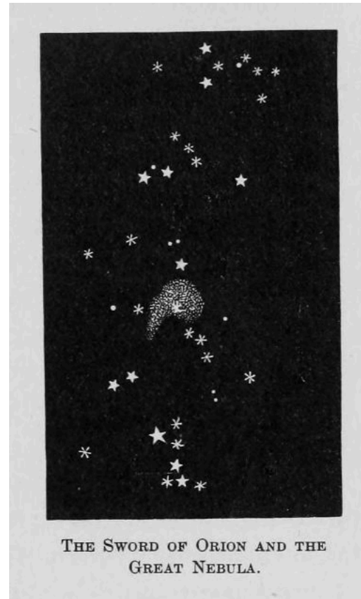
THE SWORD OF ORION AND THE GREAT NEBULA.
