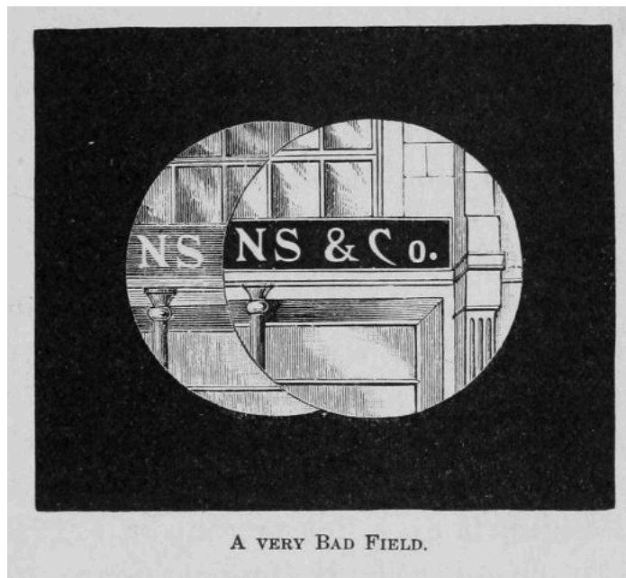
A VERY BAD FIELD.
