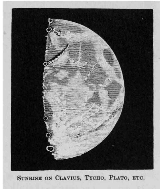
SUNRISE ON CLAVIUS, TYCHO, PLATO, ETC.
