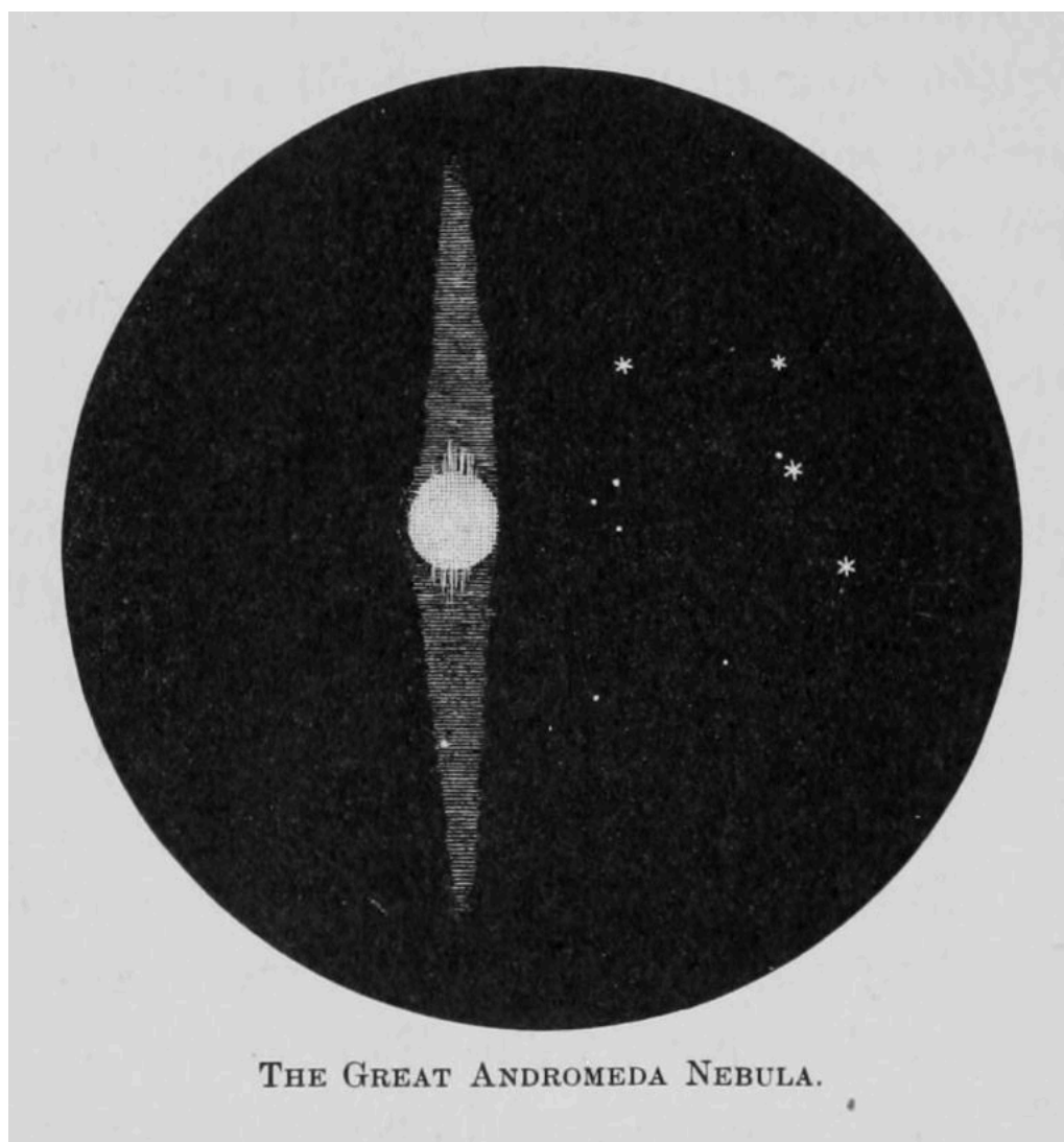
THE GREAT ANDROMEDA NEBULA.
