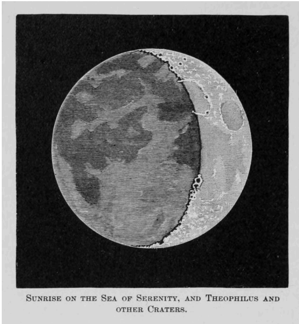
SUNRISE ON THE SEA OF SERENITY, AND THEOPHILUS AND OTHER CRATERS.
