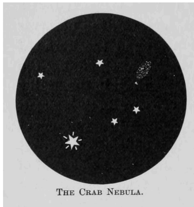
THE CRAB NEBULA.
