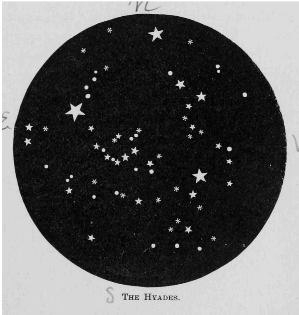
THE HYADES.
