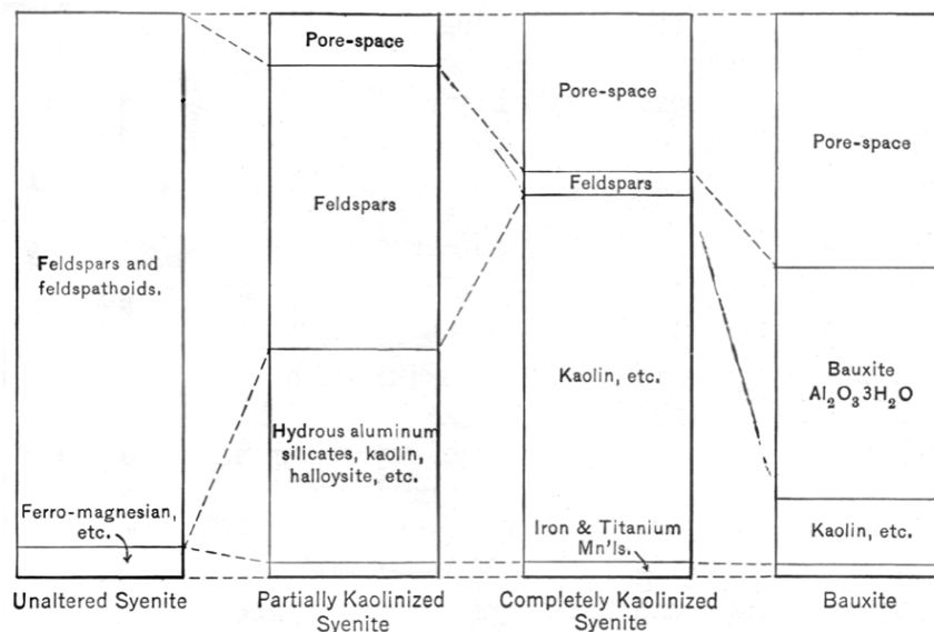
FIG. 13. Diagram showing gradation from syenite to bauxite in terms of volume. The columns represent a series of samples from a single locality in Arkansas. After Mead. ToList
