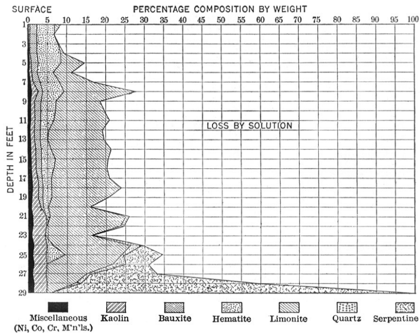
FIG. 12. Representing in terms of weight the mineralogical changes in the katamorphism of serpentine rock to iron ore, on the assumption that alumina has remained constant, eastern Cuba. ToList
