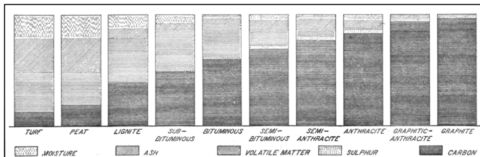
FIG. 6. Origin and development of coal. After Gilbert. ToList
