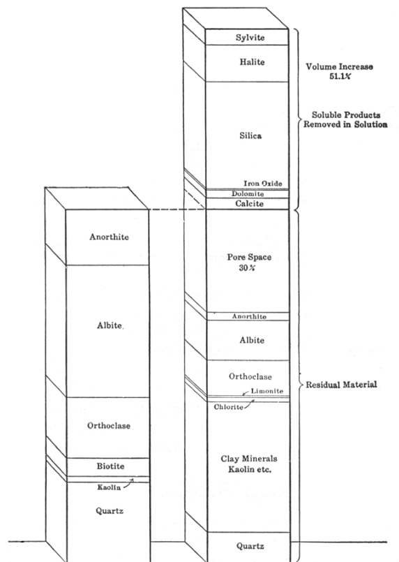
FIG. 1. Graphic representation of volume change in weathering of a Georgia granite. To List
