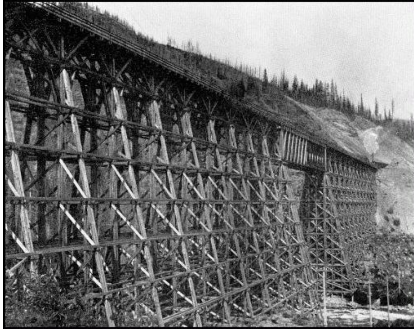
MOUNTAIN CREEK BRIDGE—Containing 1,500,000 feet timber.
