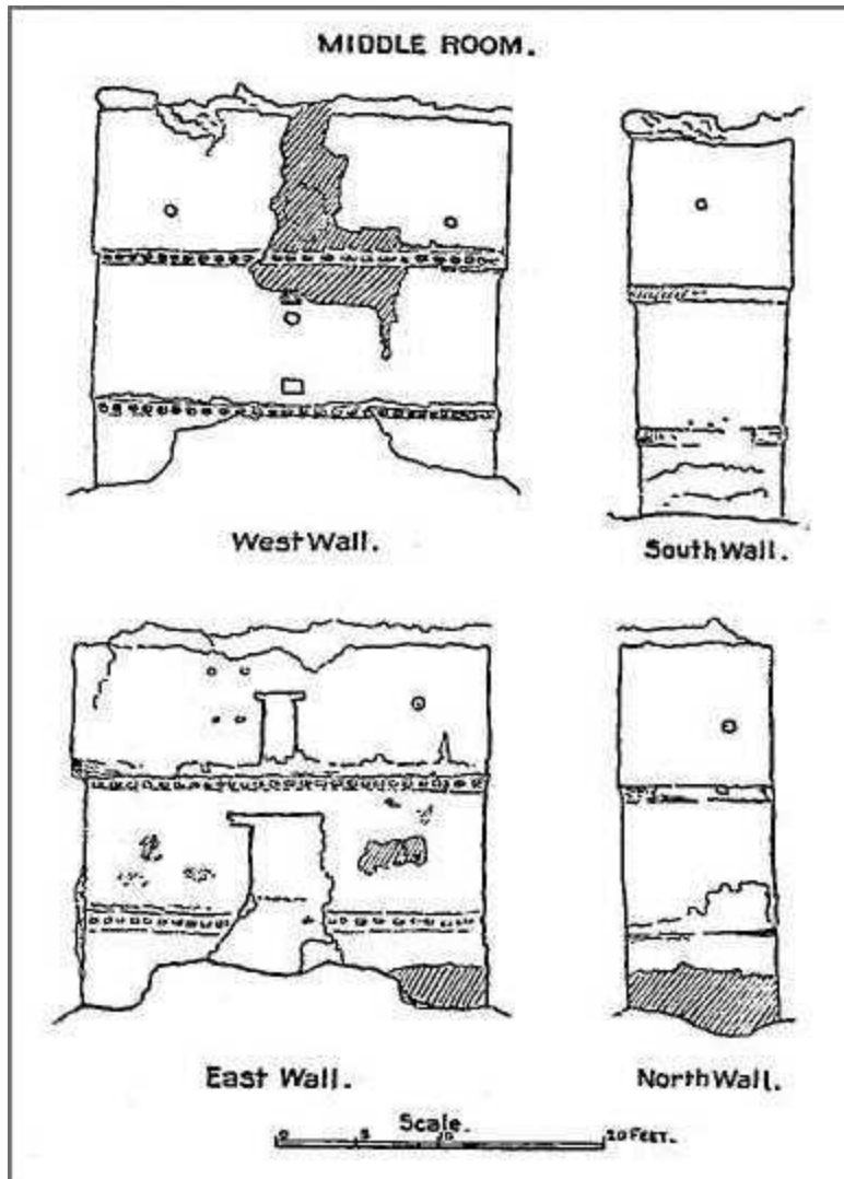
Fig. 330.—Elevations of walls, middle room.
