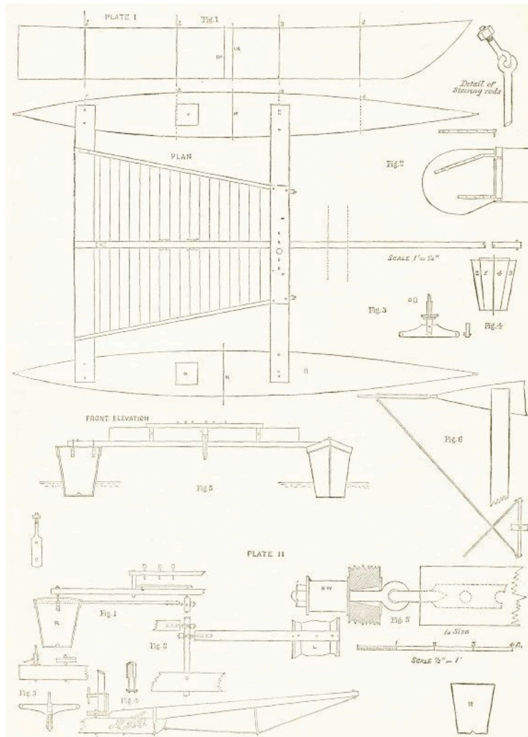
WORKING PLANS OF A CATAMARAN.
