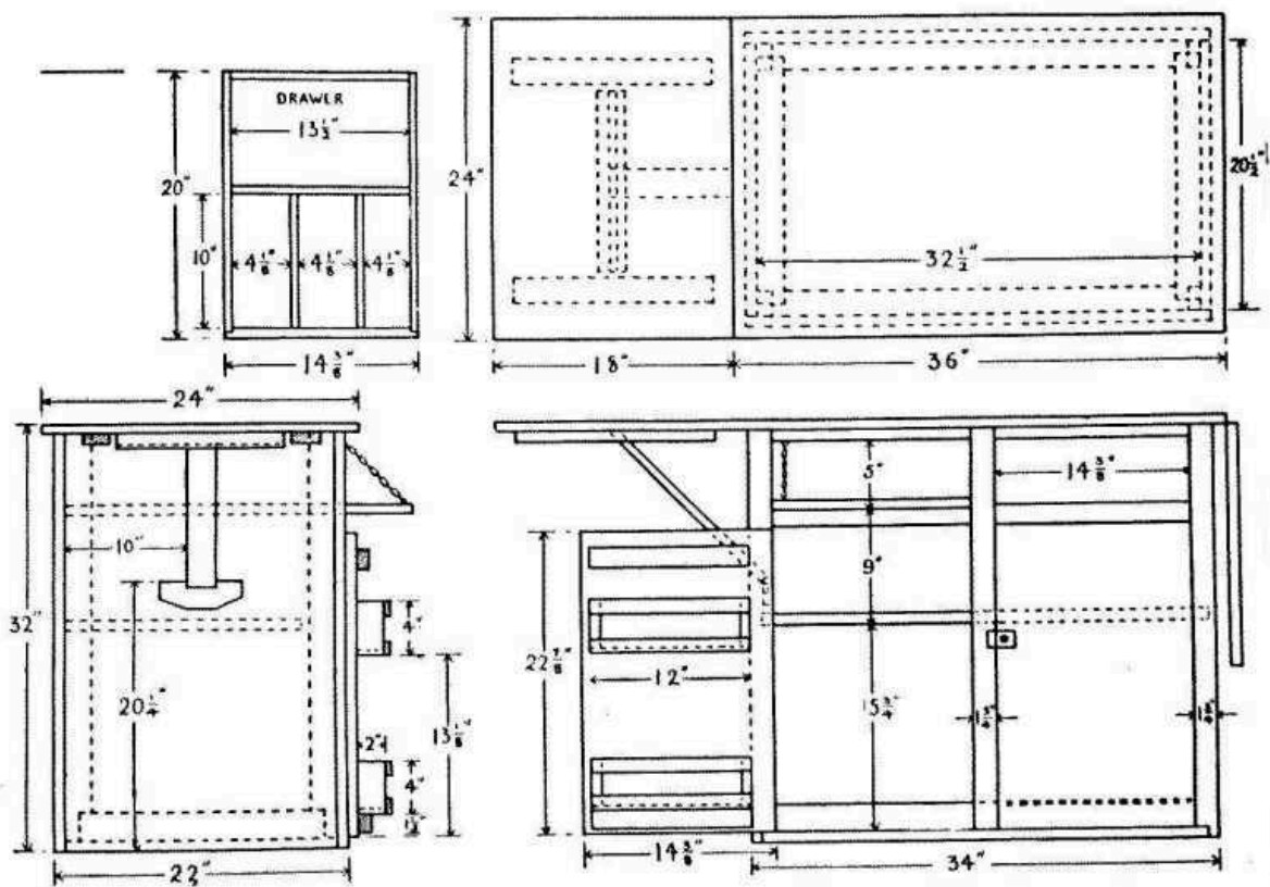
FIG. 36.—Working details
