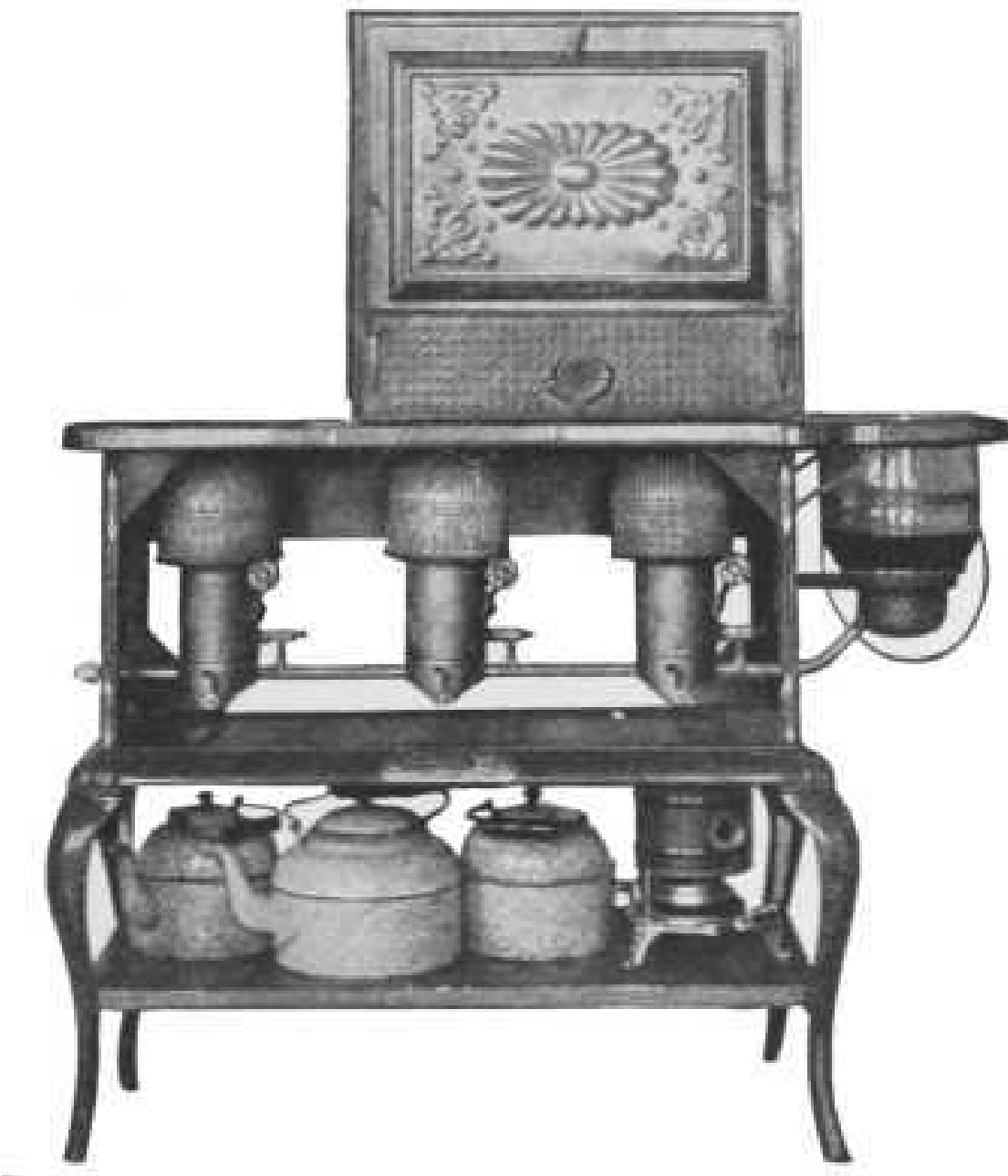
FIG. 33.—Three-flame-burner oil-stove, with kettles and one-flame-burner oil-stove on shelf
