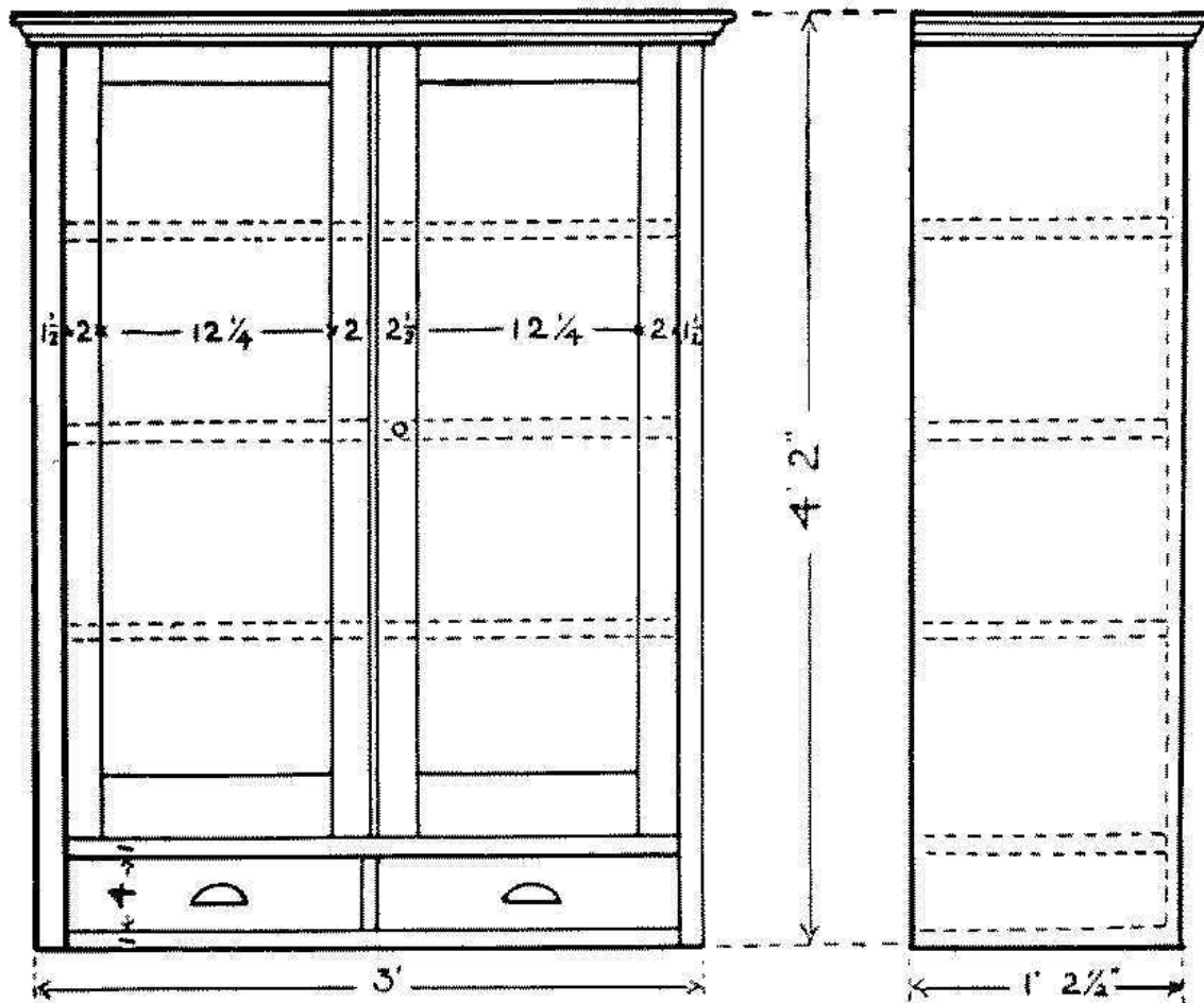
FIG. 28.—Working drawings of cupboard
