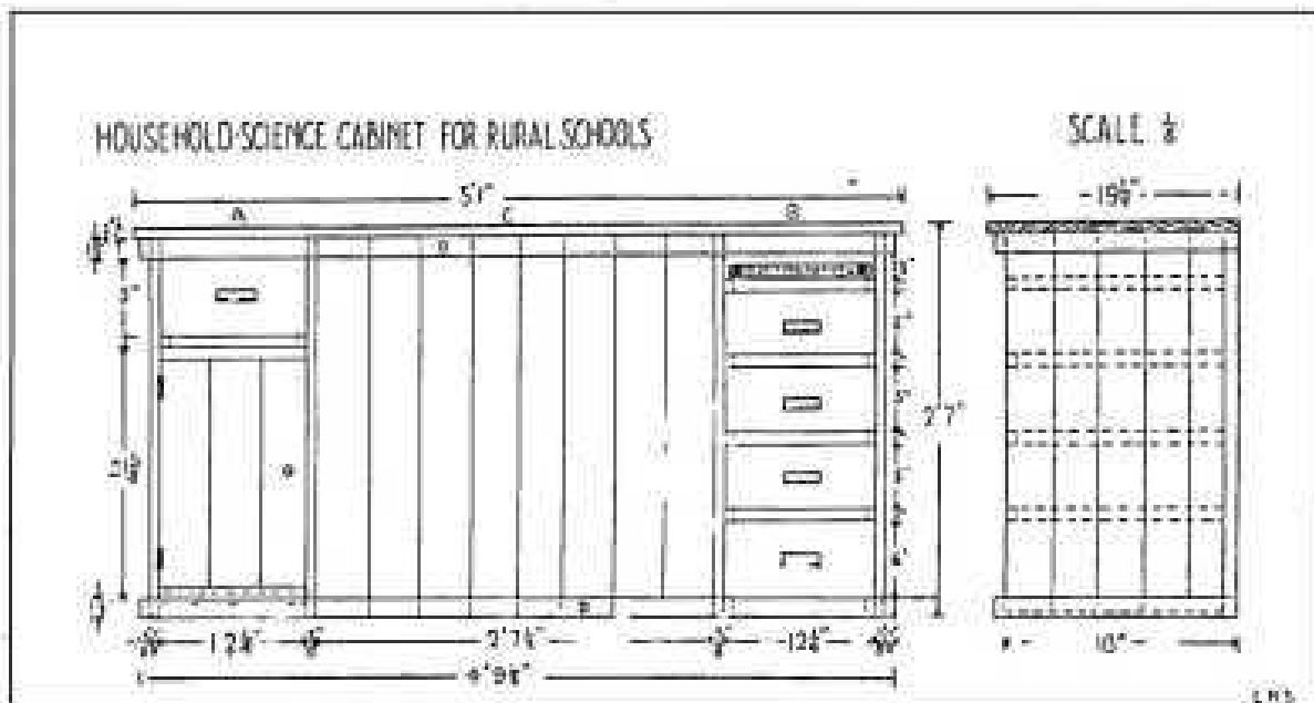
FIG. 24—Household Science Cabinet for Rural Schools
