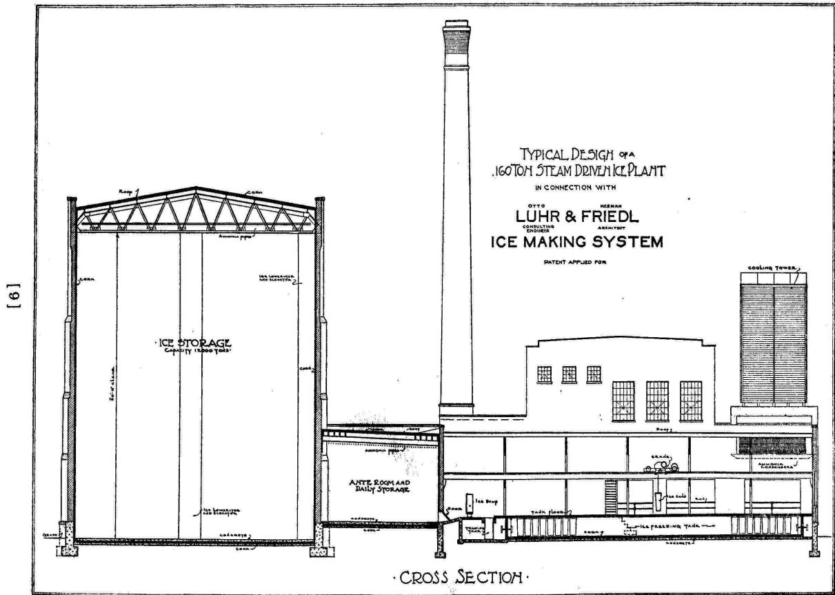
Typical Design of a 160 Ton Steam Driven Ice Plant. Exterior Cross Section In connection with Otto Luhr Consulting Engineer & Herman Fridel Architect Ice Making System Patent Applied For
