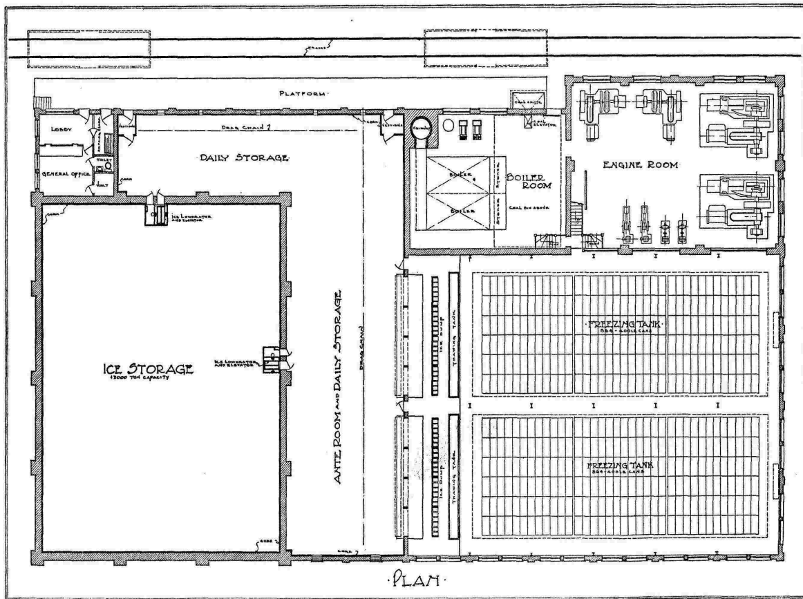
Typical Design of a 160 Ton Steam Driven Ice Plant. Interior Details
