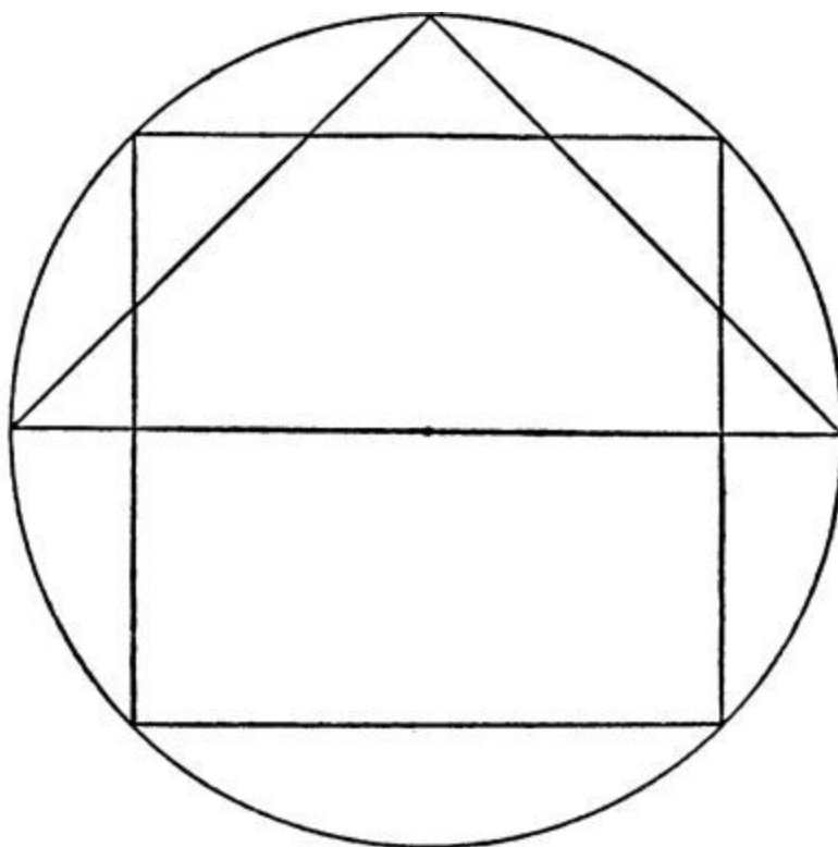
FIG. 19.—Kosmic Pentoglyph
