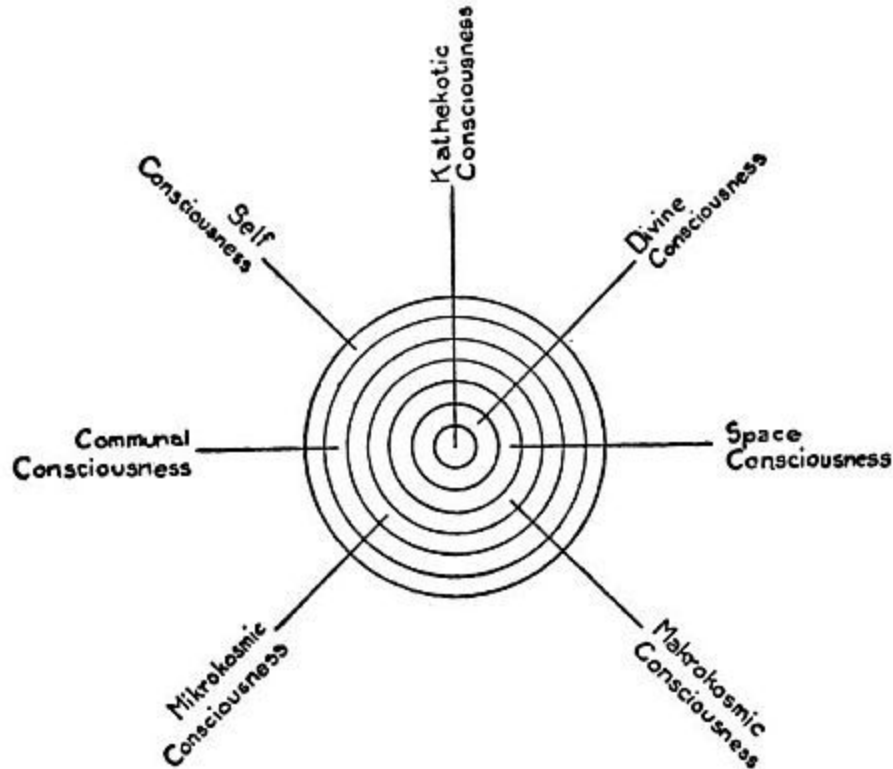
FIG. 21.—Septenary Enveilment of Consciousness
