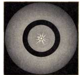
WONDERFUL NEBULA IN GEMINI (1532).
