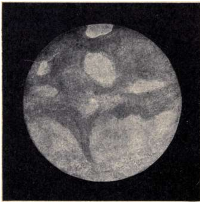
MARS SEEN WITH A FIVE-INCH TELESCOPE.
