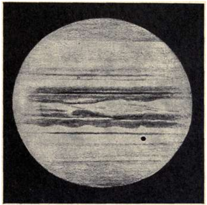
JUPITER SEEN WITH A FIVE-INCH TELESCOPE.
