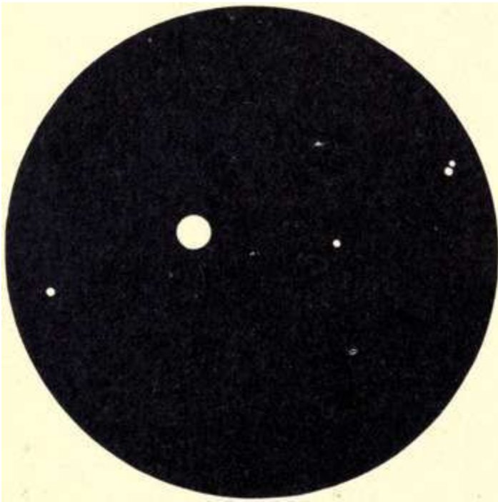
PROCYON AND ITS NEIGHBORS.
