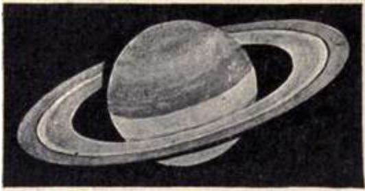
SATURN SEEN WITH A FIVE-INCH TELESCOPE.
