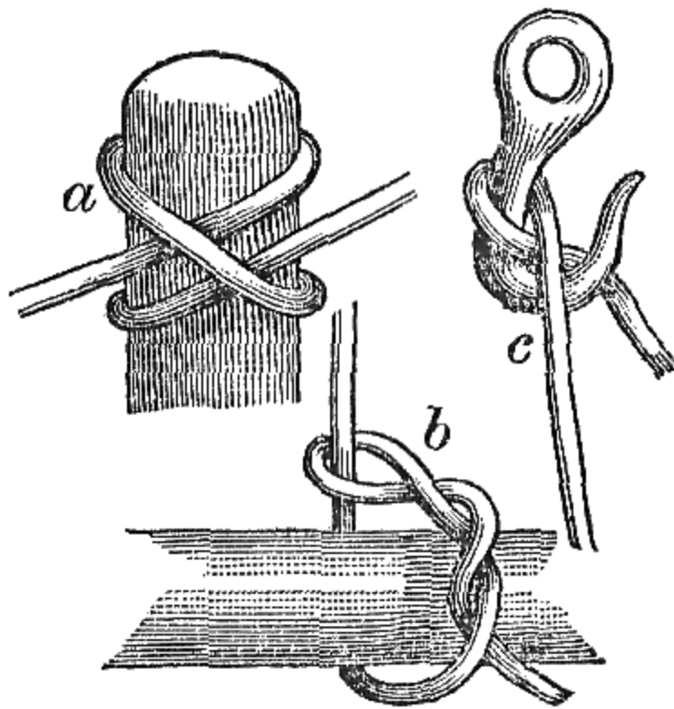
a , Clove-hitch; b , Timber-hitch; c , Blackwall-hitch.
