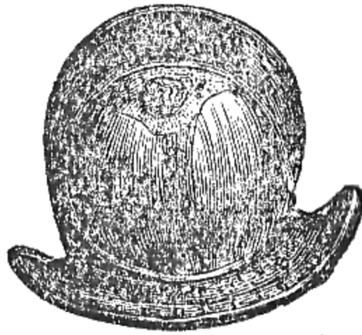
Morion.
