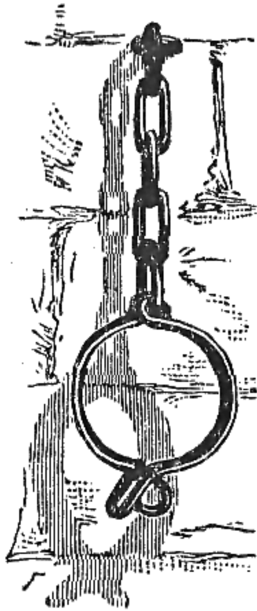
Jougs.
