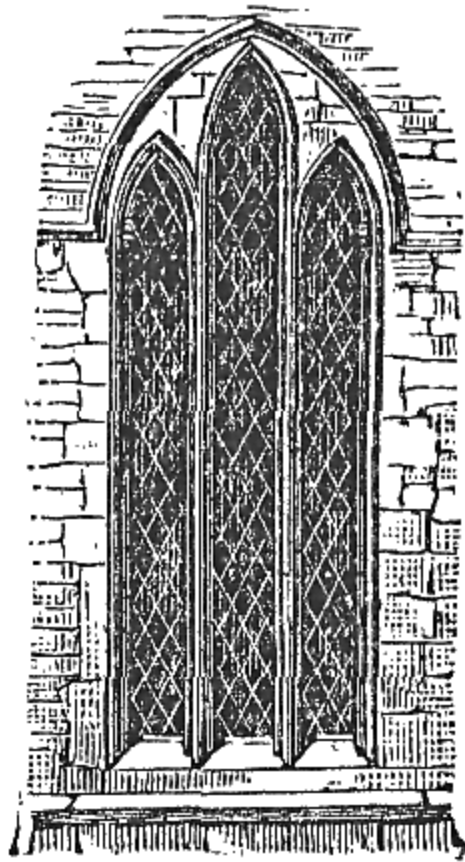
Lancet Window.
