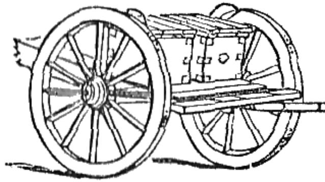
Limber.
