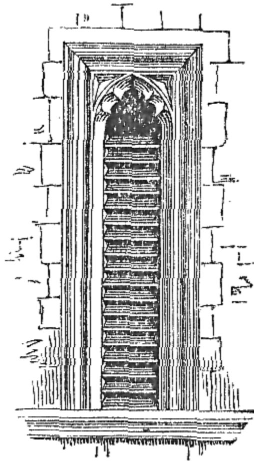
Louvre-window.
