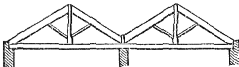
M-roof.
