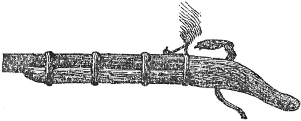
Matchlock.
