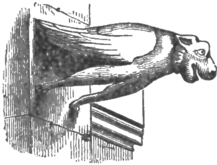
Gargoyle.
