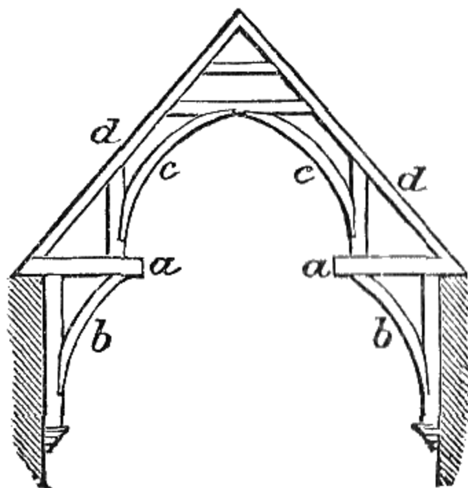
Section of Hammer- beam Roof:
