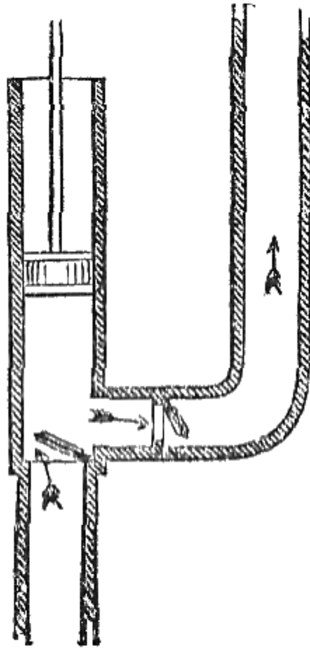
Section of Force-pump.
