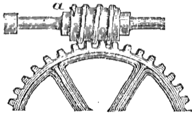
a , Endless Screw.
