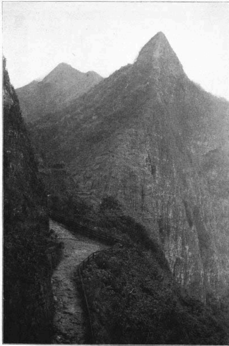
Scene in Olokele Gulch, Makaweli, Kauai.
