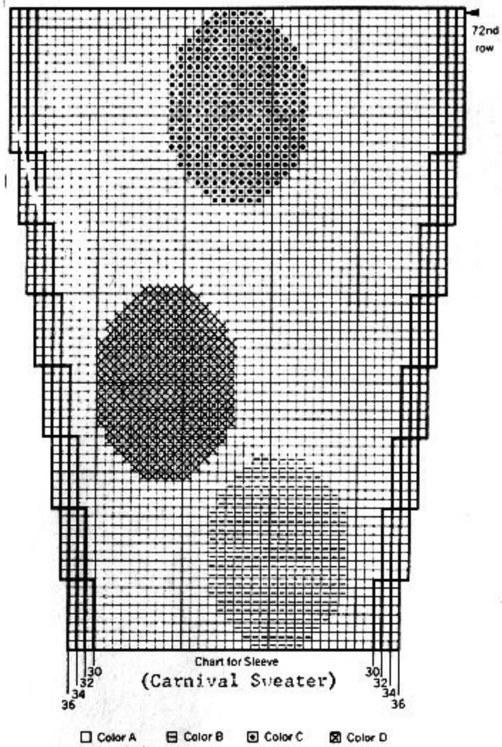
Chart for Sleeve (Carnival Sweater)
