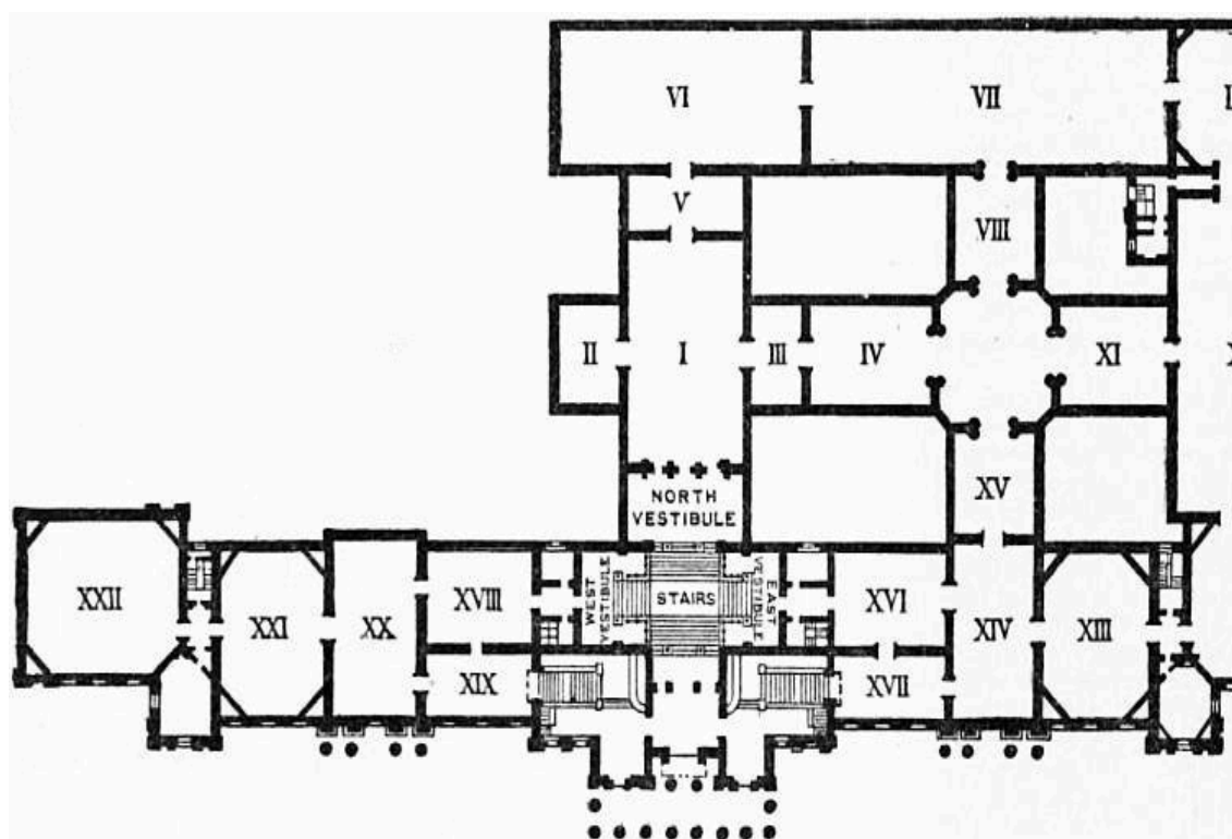
FIG. 1.—Plan of the National Gallery, London.
