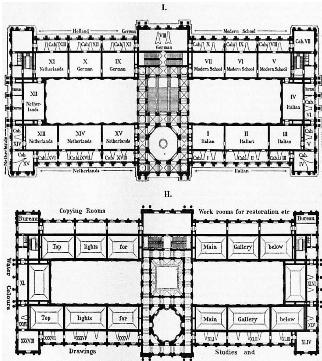
FIG. 2.—Plan of the first and second floors of the Imperial Gallery, Vienna.
