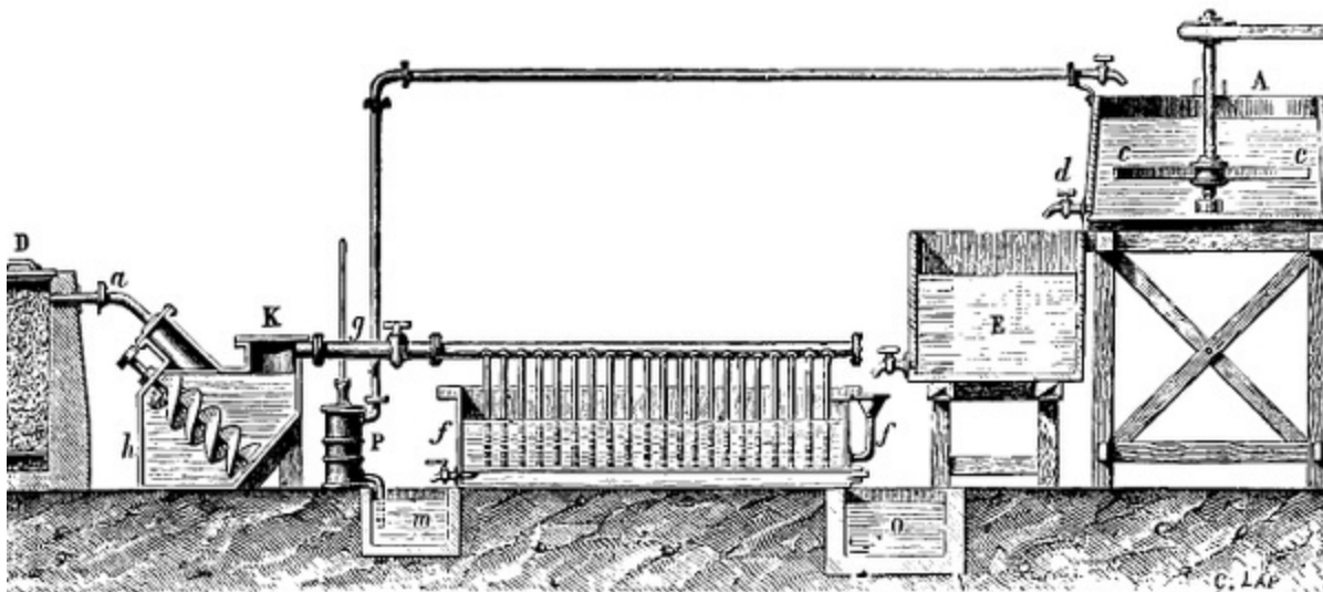
FIG. 82.—Manufacture of white lead.
