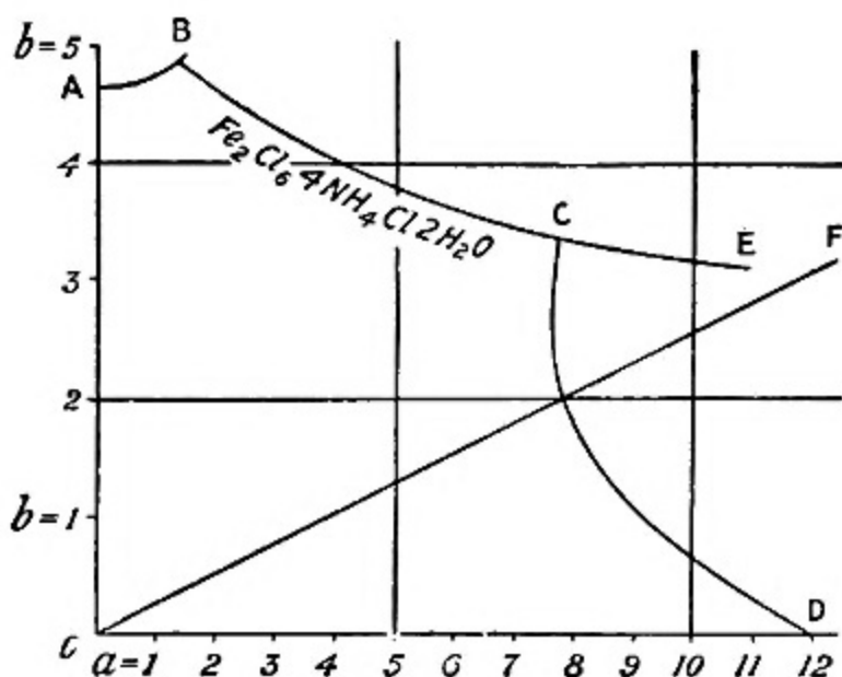
FIG. 96.—Diagram of the formation, at 15°, of the double salt \text{Fe}_2\text{Cl}_6\cdot 4\text{NH}_4\text{Cl}\cdot 2\text{H}_2\text{O} or \text{Fe}(\text{NH}_4)_2\text{Cl}_5\text{H}_2\text{O} . (After Roozeboom.)
