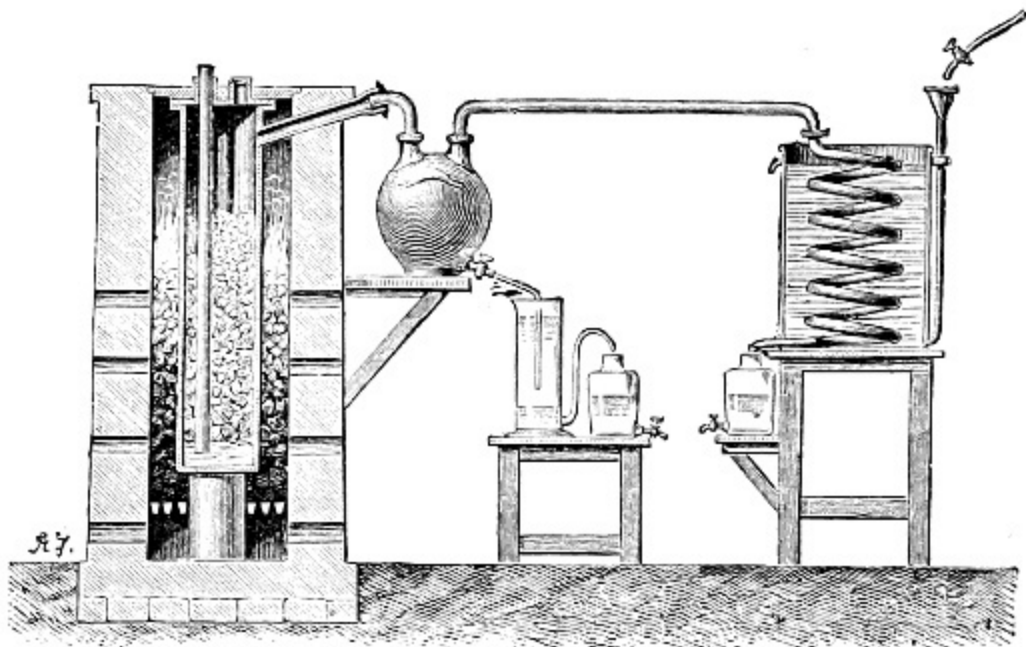
FIG. 90.—Apparatus for the manufacture of carbon bisulphide.
