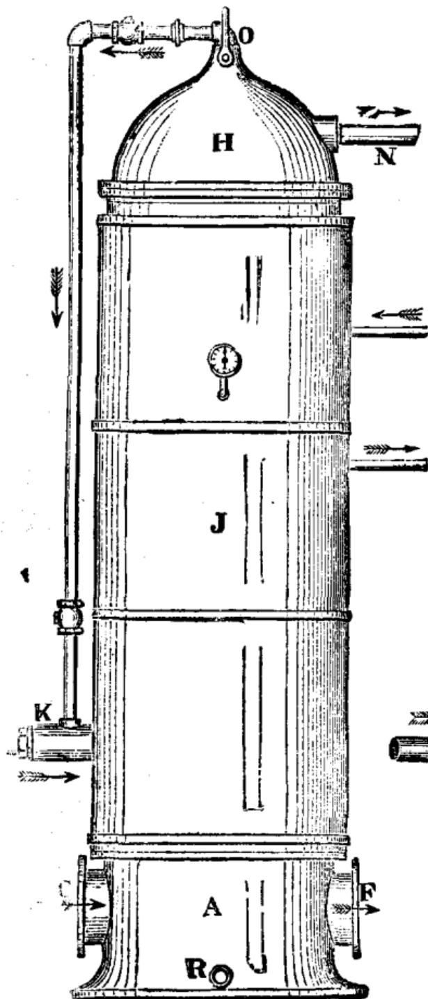
FIG. 1.—Elevation.
