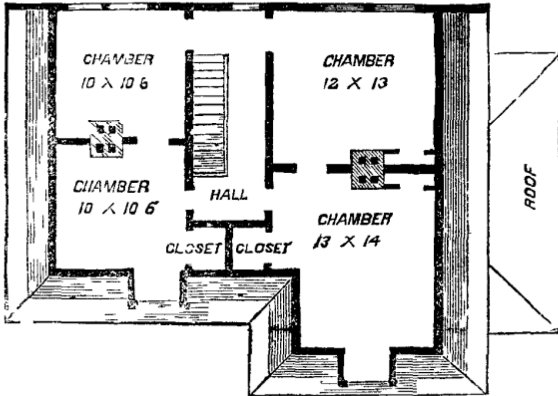
A MANSARD ROOF DWELLING. Second Floor.
