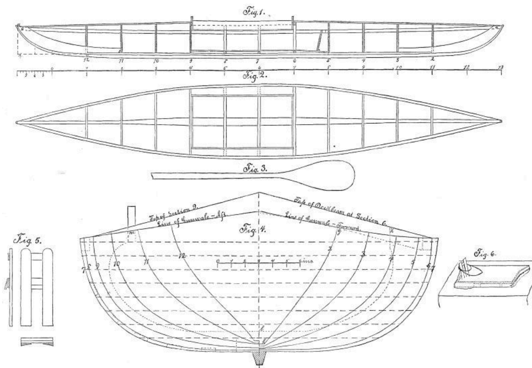
WORKING PLANS FOR A CANVAS CANOE.—[See Pages 350 and 351.]
