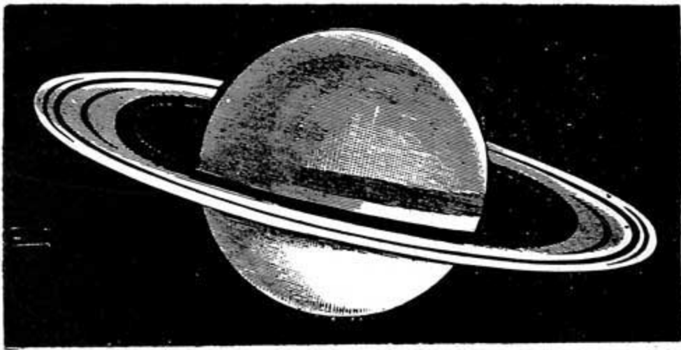
THE RINGED PLANET SATURN.
