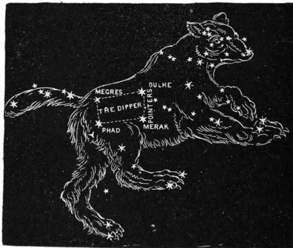
THE GREAT BEAR.
