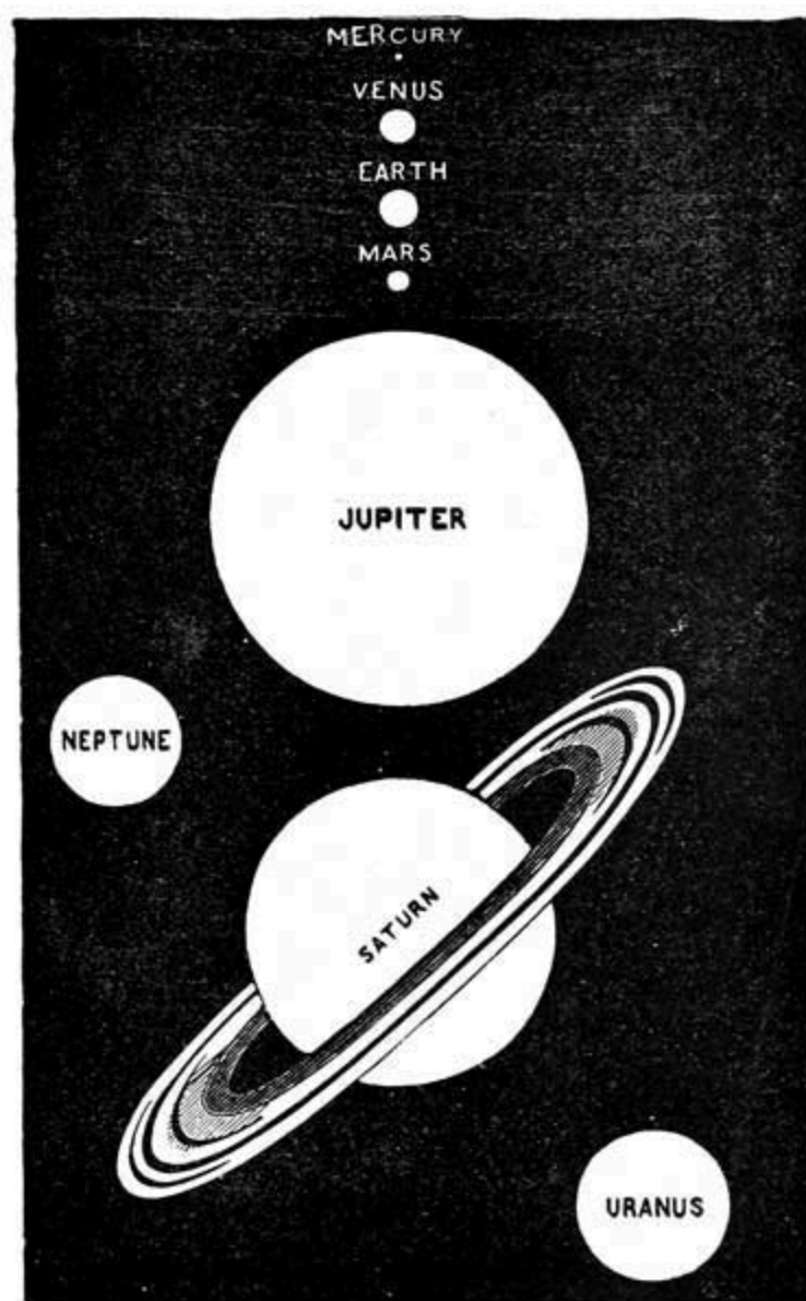
COMPARATIVE SIZE OF THE PLANETS.
