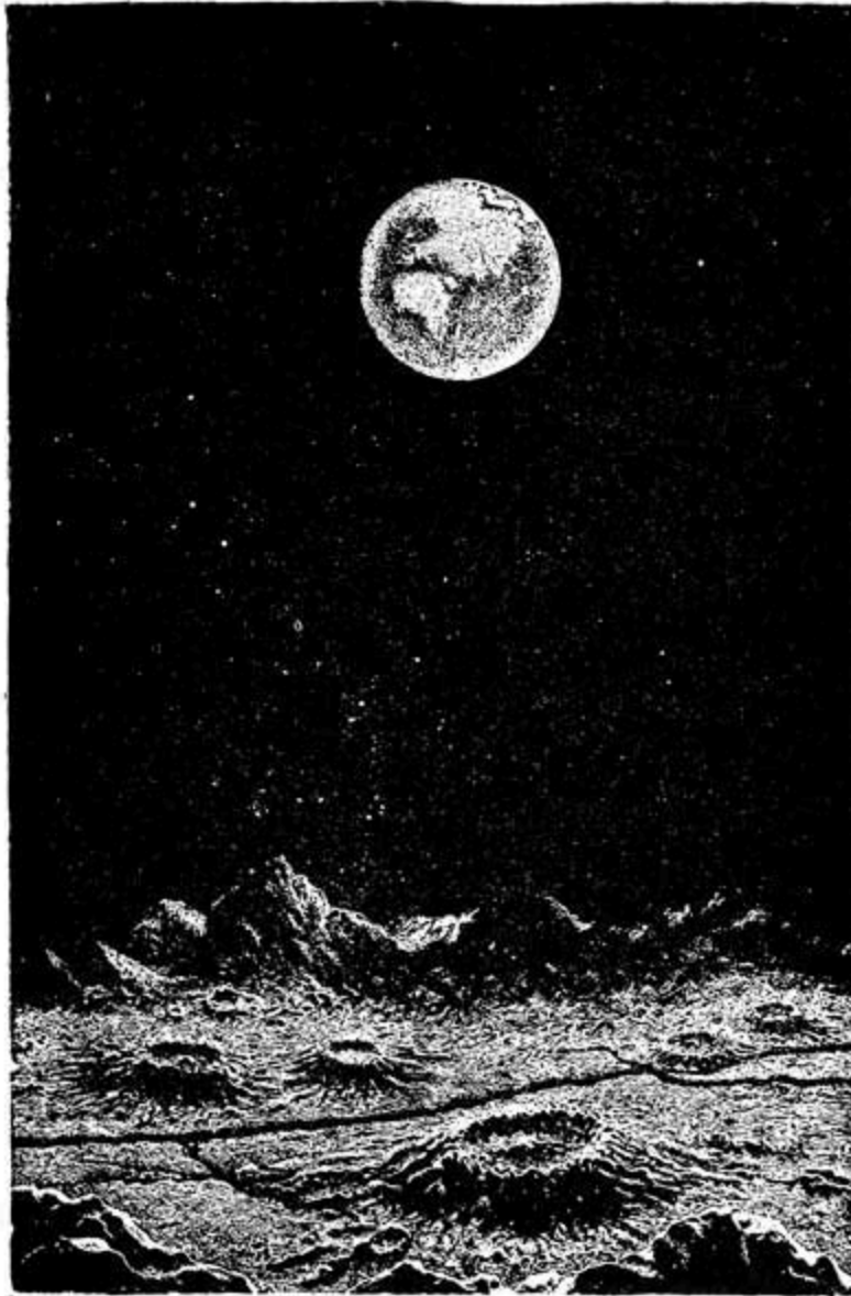
EARTH AS SEEN FROM THE MOON.
