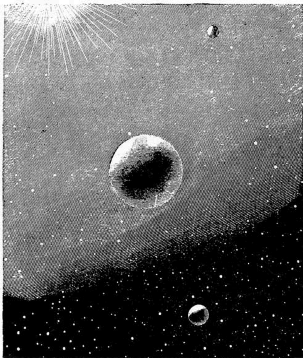
EARTH IN SPACE.
