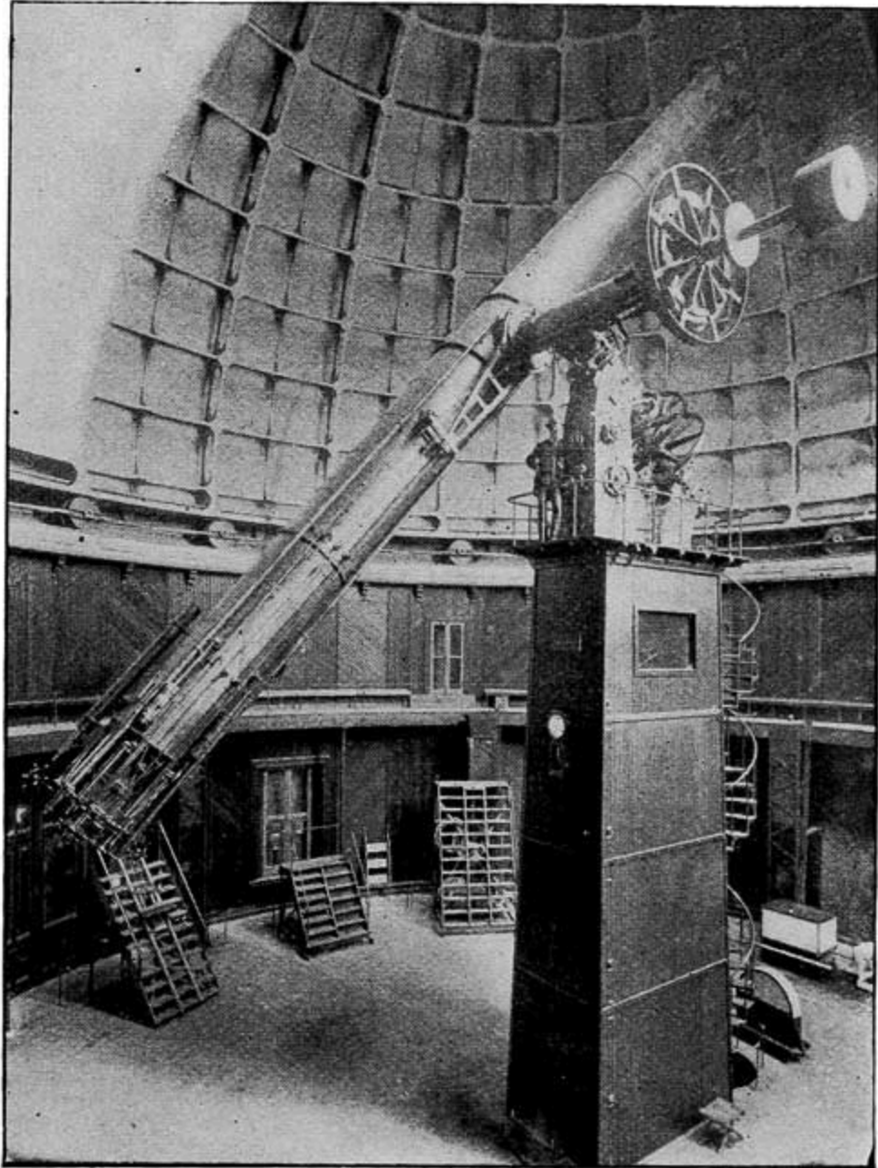
THE GREAT TELESCOPE AT LICK OBSERVATORY.
