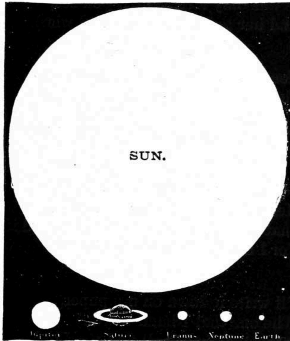
SIZE OF PLANETS, COMPARED WITH THE SUN.
