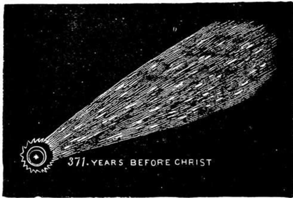
OLD PICTURE OF A COMET.
