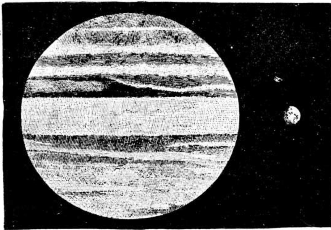
GIANT JUPITER AND THE EARTH.
