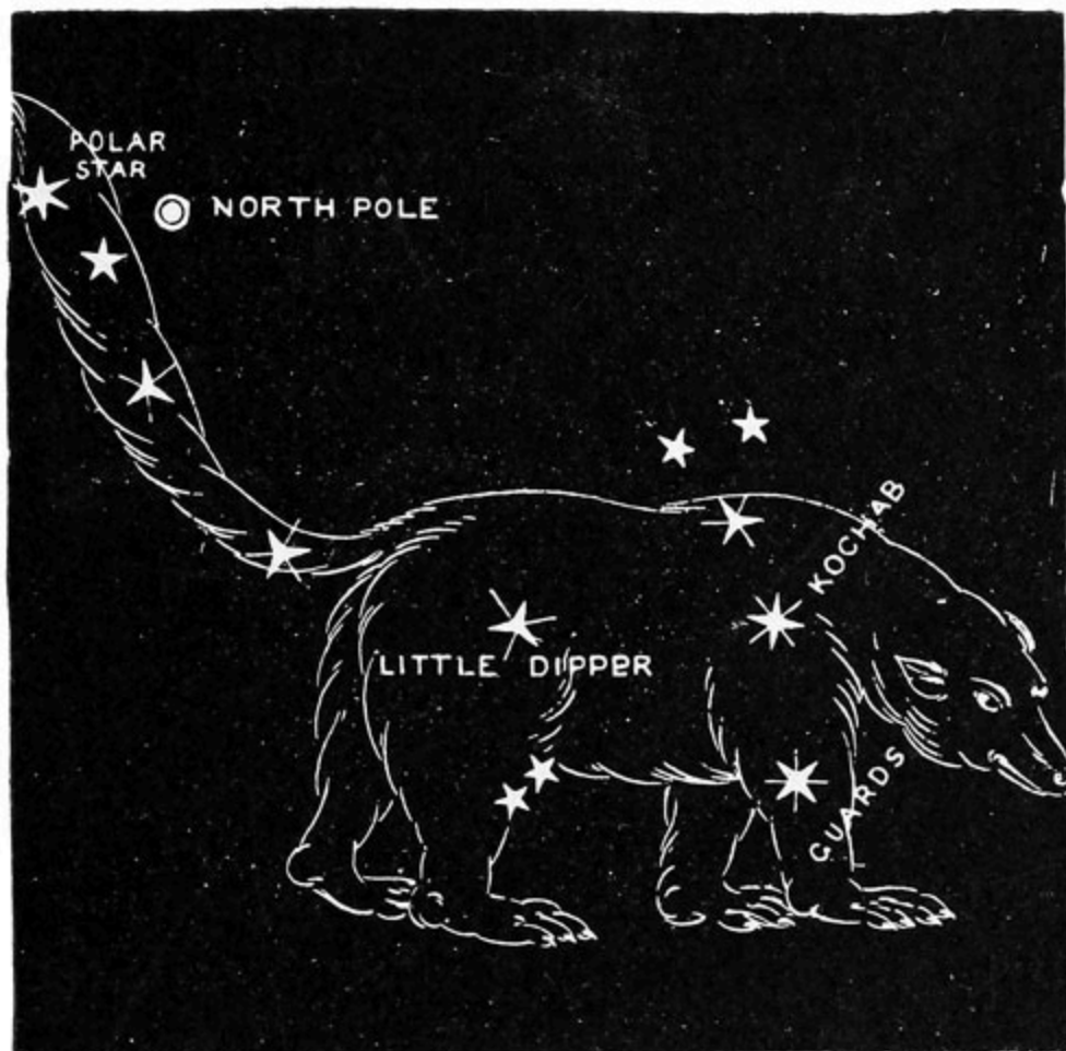
THE LITTLE BEAR.
