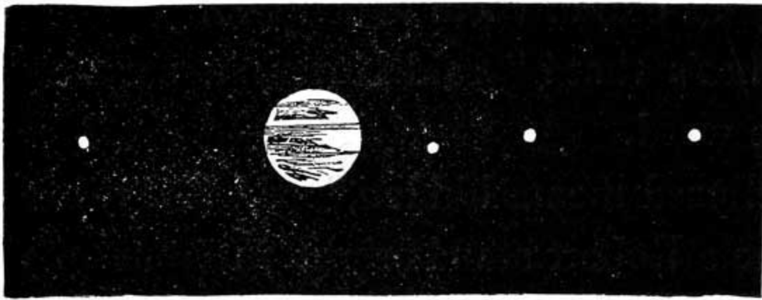
JUPITER AND HIS MOONS.
