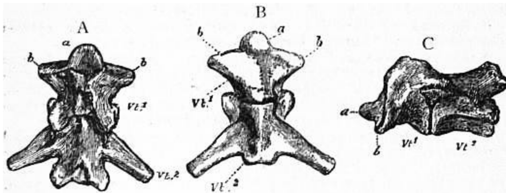
FIG. 4.—The first two vertebrae of Necturus . Vt1 , Atlas; Vt2 , second vertebrae; a , intercondyloid process of the atlas; b , the articular surfaces for the occipital condyles. The ribs of the second vertebra are not represented. A, Dorsal; B, ventral; C, lateral view.
