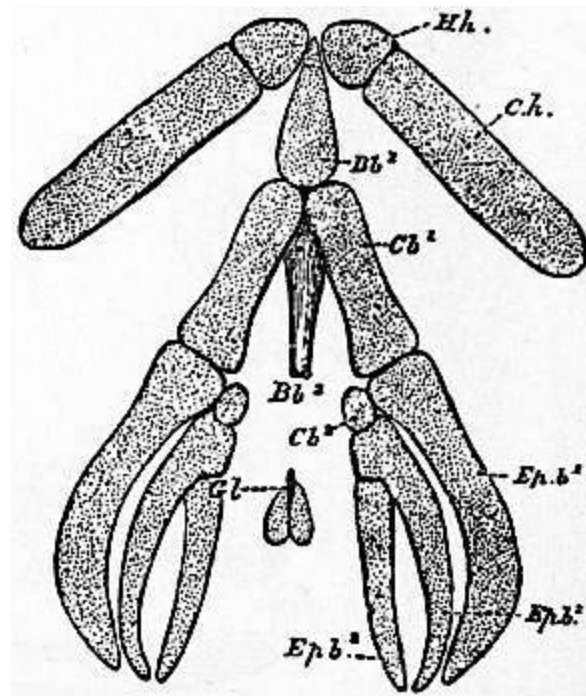
FIG. 11.—Hyoid and branchial apparatus of Necturus maculosus .
