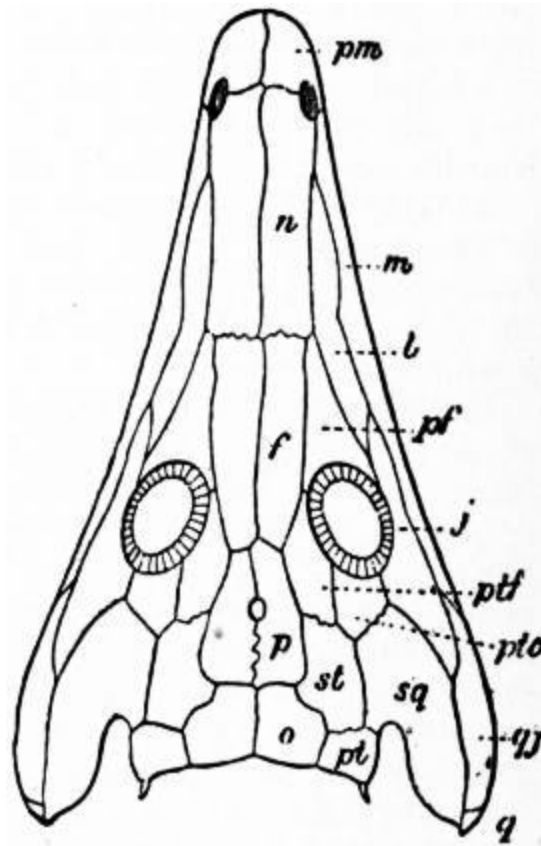
FIG. 1.—Upper view of Archegosaurus Decheni .
