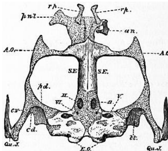
FIG. 7.—Chondrocranium of Rana esculenta —ventral aspect.
