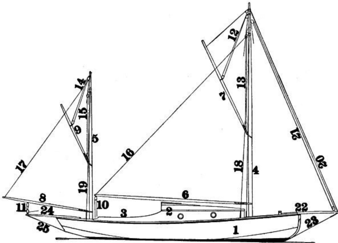
SPAR AND RIGGING PLAN OF YAWL.
