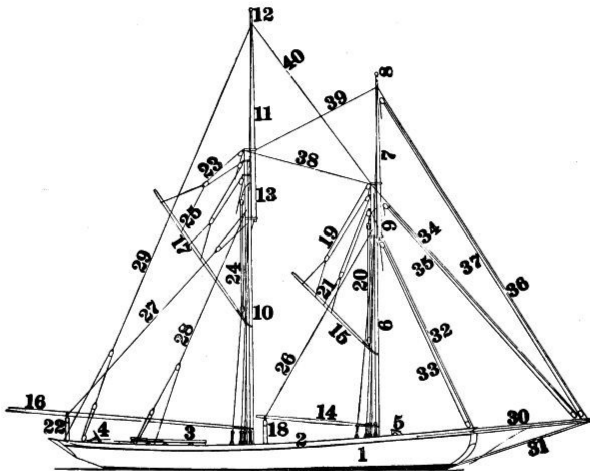
SPAR AND RIGGING PLAN OF SCHOONER.
