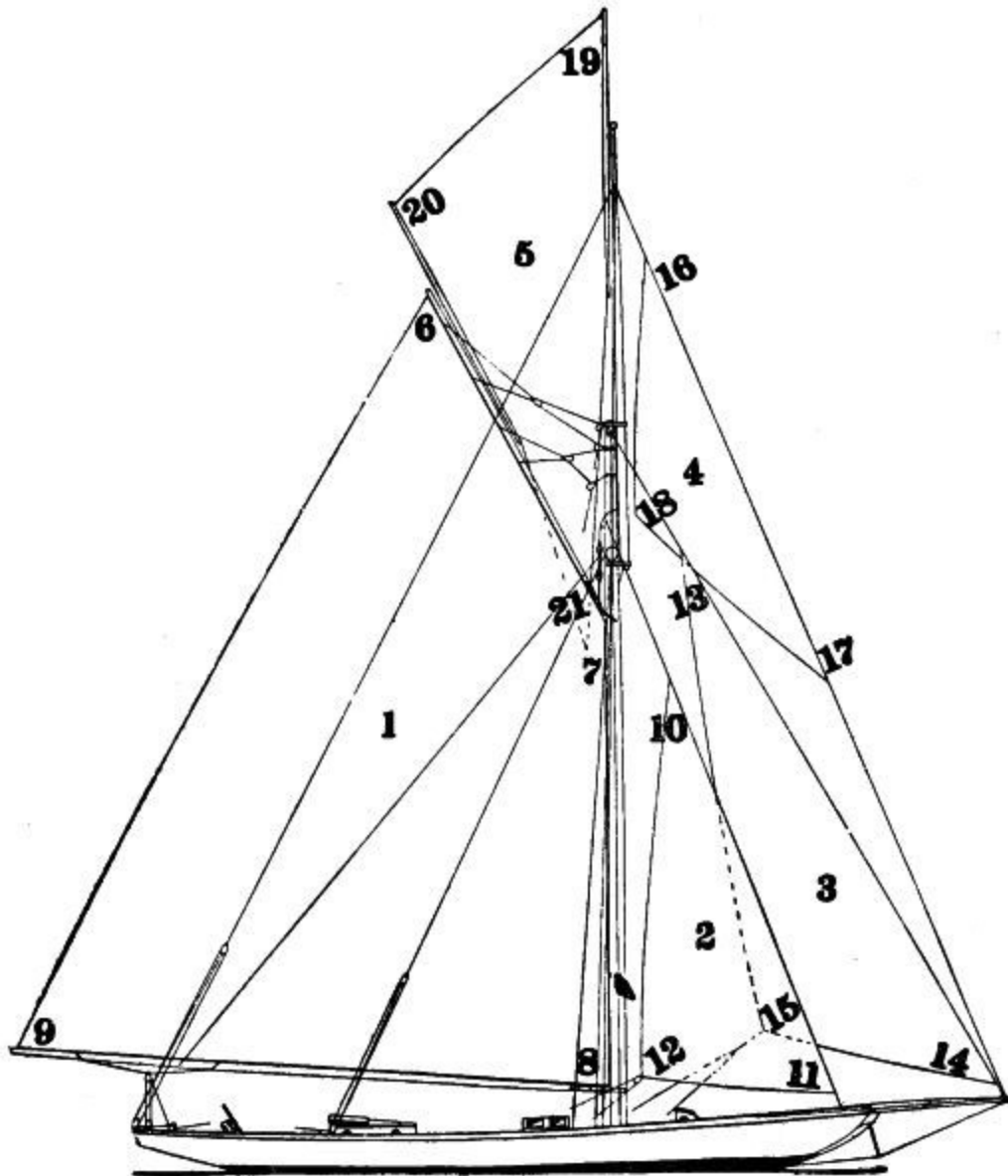
SAIL PLAN OF TOPSAIL SLOOP.
