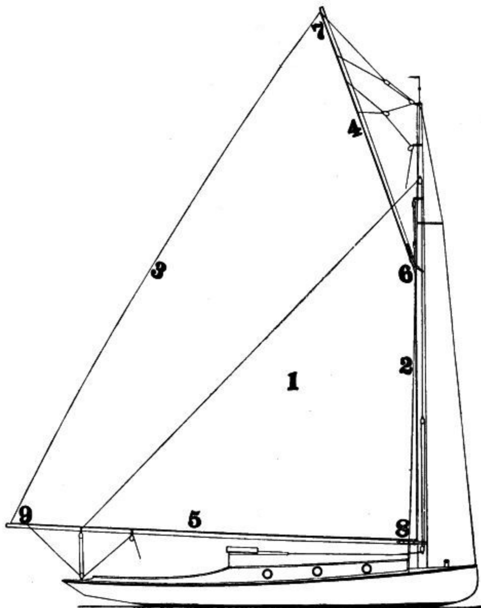
SAIL PLAN OF CAT BOAT.
