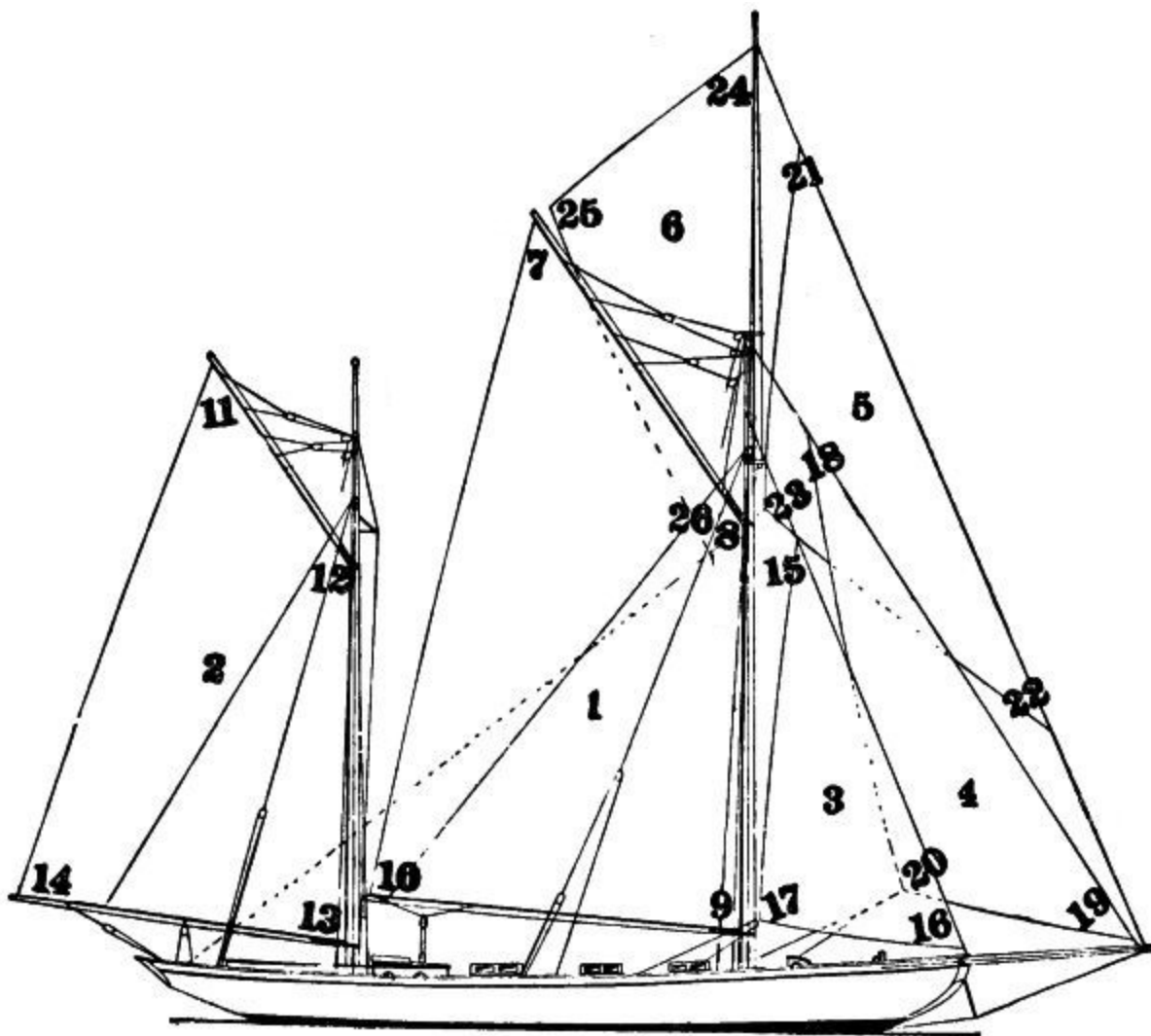
SAIL PLAN OF KETCH.
