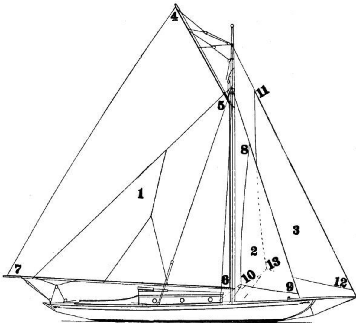
SAIL PLAN OF POLE MAST SLOOP.
