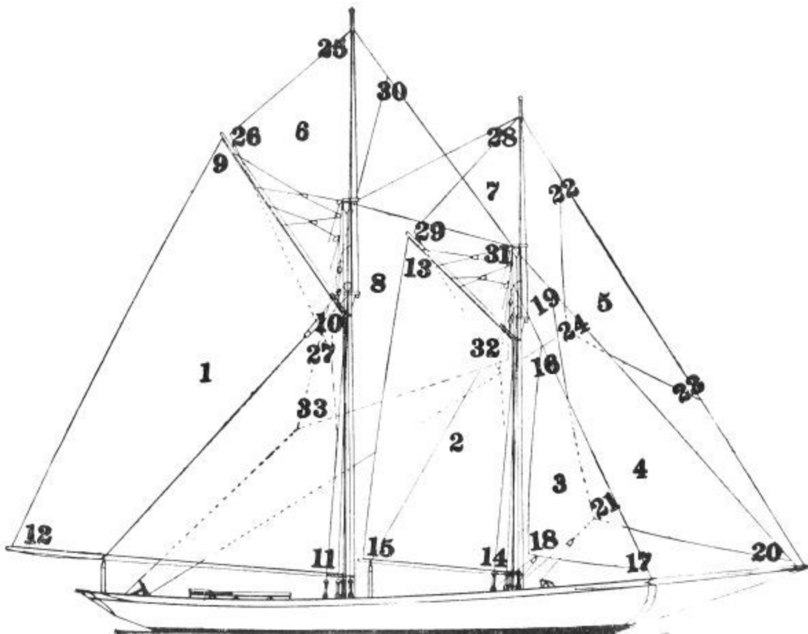
SAIL PLAN OF SCHOONER.
