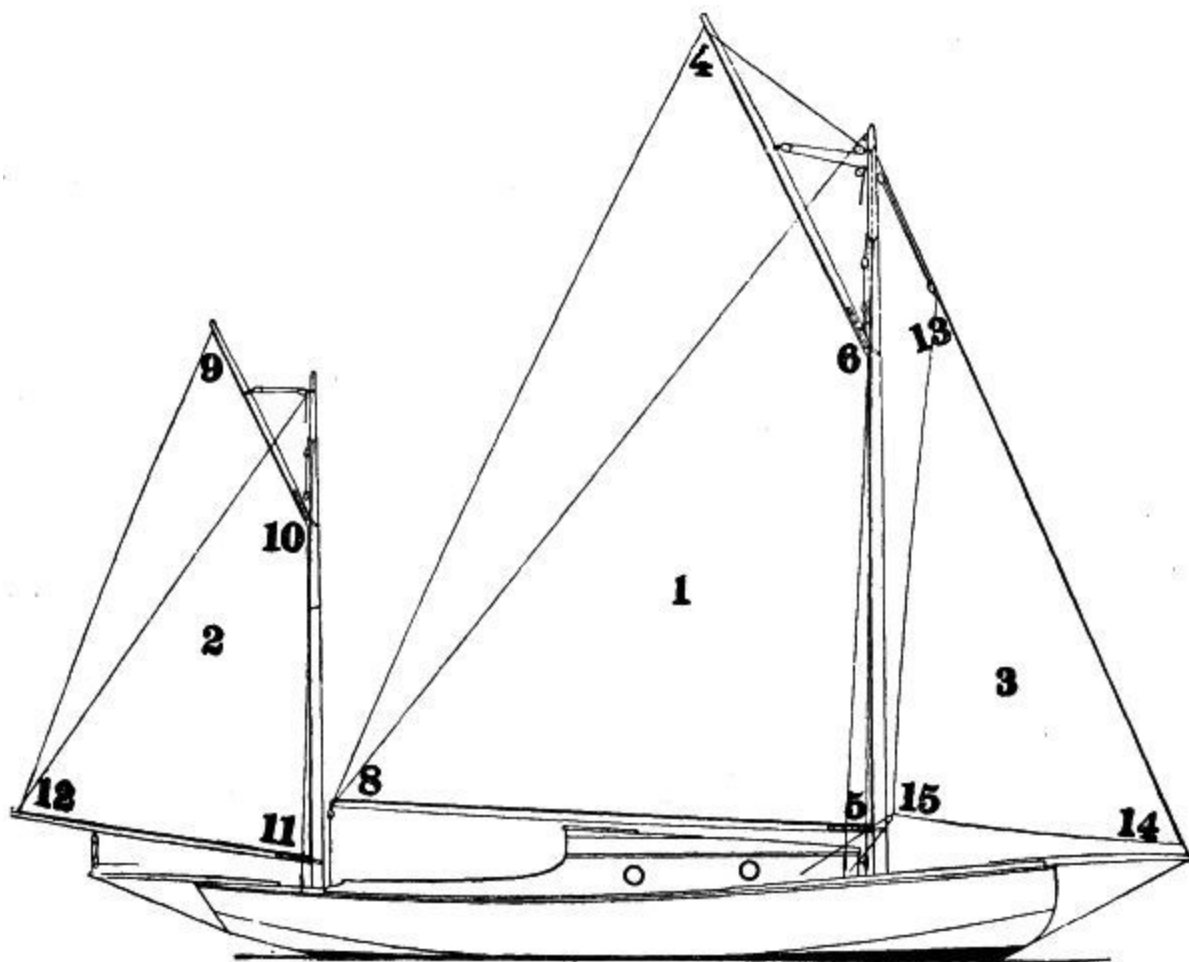
SAIL PLAN OF YAWL.
