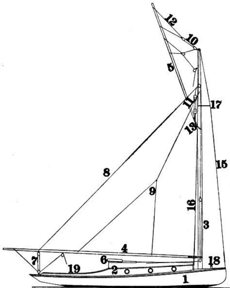
SPAR AND RIGGING PLAN OF CAT BOAT.
