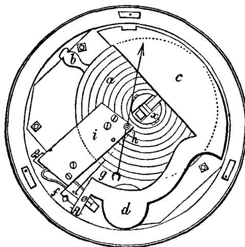
FIG. 4.—Aneroid Barometer.
