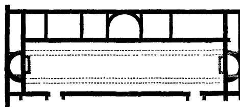
FIG. 7.—Plan of Basilica adjoining the Forum of the Roman city at Silchester, Hants. (From Archaeologia , vol. liii.)
