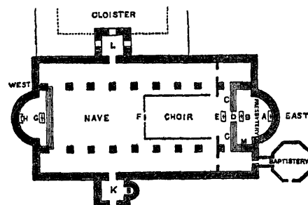
FIG. 22.—Ground-Plan of the original Cathedral at Canterbury, as restored by Willis. A, High altar. B, Altar of our Lord. C, C, Steps to crypt. D, Crypt. E, F, Chorus
