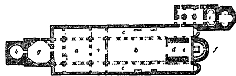
FIG. 19.—Ground-Plan of Cathedral of Parenzo, Istria.
