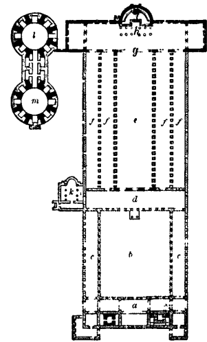
FIG. 10.—Ground-Plan of the original Basilica of St Peter's at Rome. a, Porch. b, Atrium. c, Cloisters. d, Narthex. e, Nave. f, f, Aisles. g, Bema. h, Altar, protected by a double screen. i, Bishop's throne in centre of the apse. k, Sacristy. l, Tomb of Honorius. m, Church of St Andrew.
