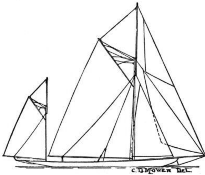
YAWL RIGS
