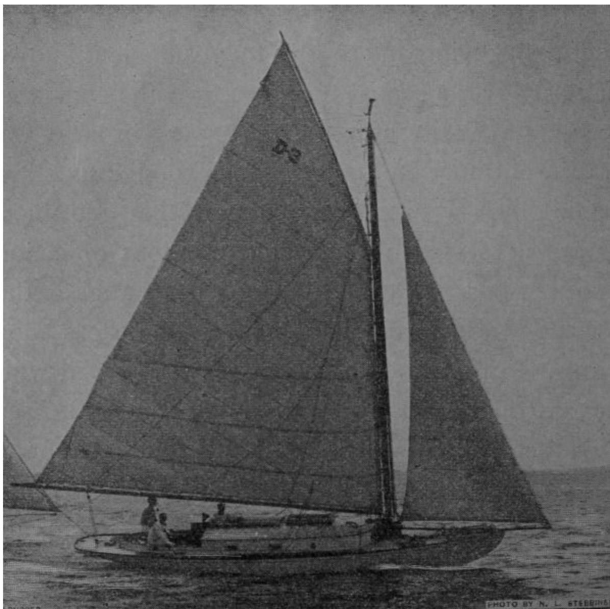
JIB AND MAINSAIL CRUISING BOAT
