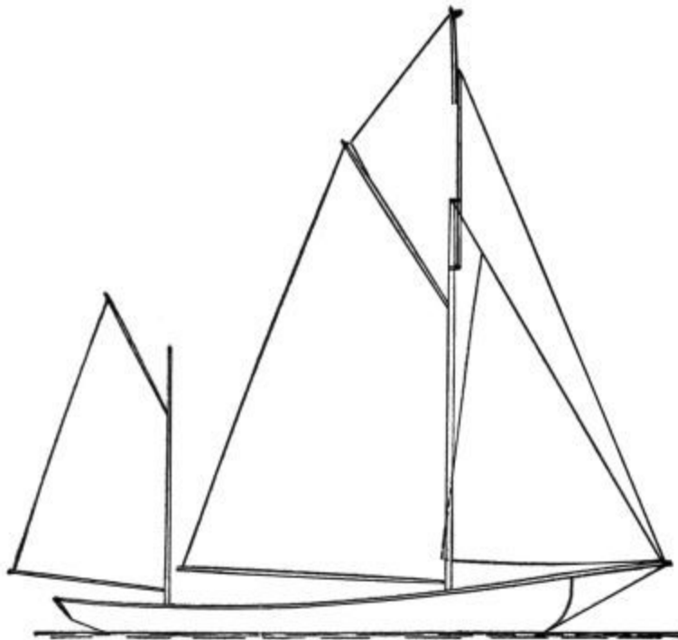
KETCH
