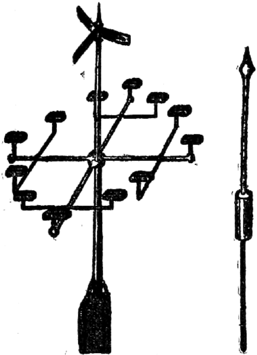
Fig. 19 (Left) and Fig. 20 (Right) The Divisch Lightning Conductor
