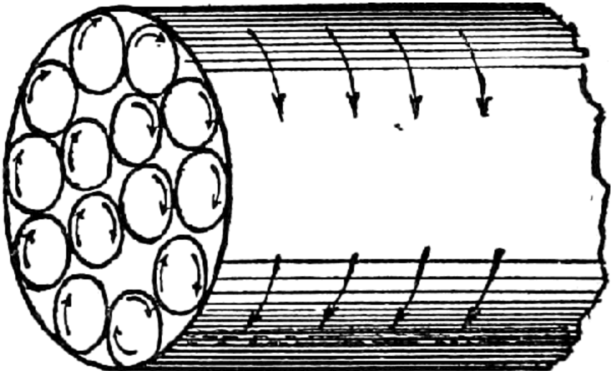
Fig. 25 Ampère's Molecular Currents
