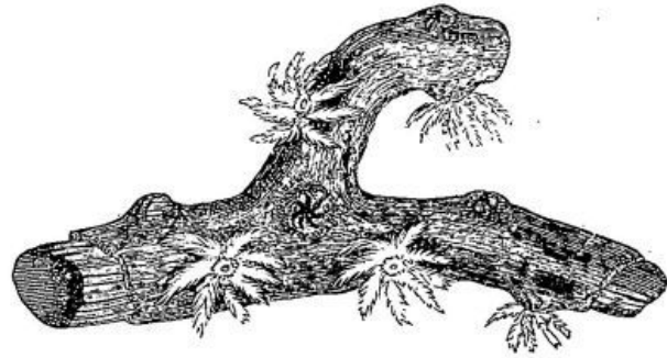
Fig. 4.—FRAGMENT OF RED CORAL WITH POLYPS.
