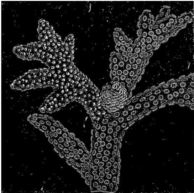
Fig. 1.—BRANCHING CORAL ALIVE, WITH POLYPS EXPANDED.
