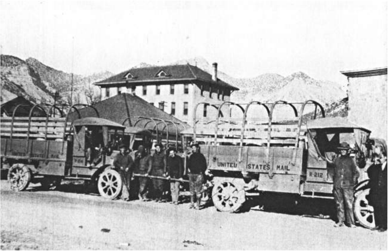
EQUIPMENT OF A POSTAL MOTOR TRUCK ROUTE
