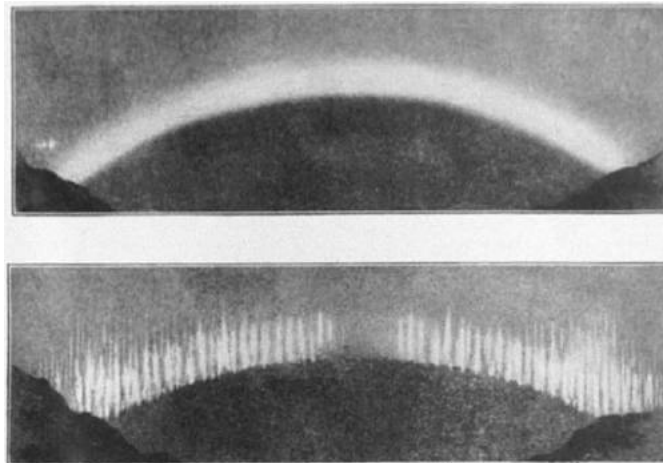
FIG. 1—TWO TYPES OF AURORAL ARCS.
