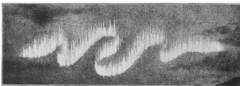
FIG. 3—AURORAL BANDS.
