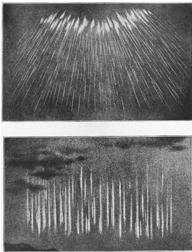
FIG. 2—TWO TYPES OF AURORAL RAYS.
