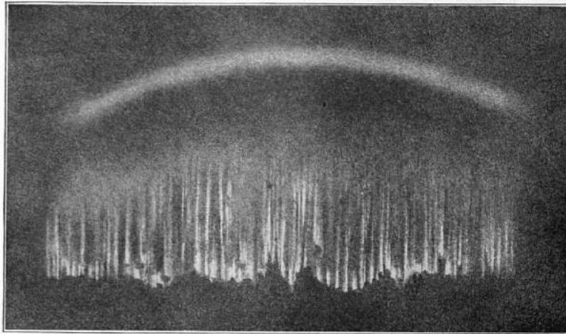
FIG. 4—AURORAL CURTAIN BELOW AN ARC.
