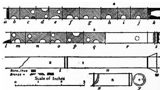
FIG. 1.—Diagram of the Fragments of an Aulos (Candia Mus.).
