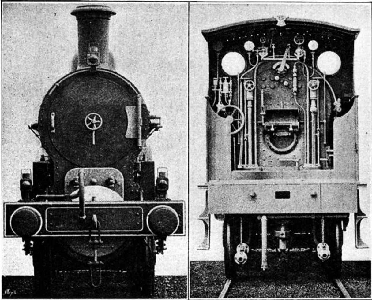
BACK AND FRONT VIEW OF THE LOCOMOTIVE "GREATER BRITAIN."
