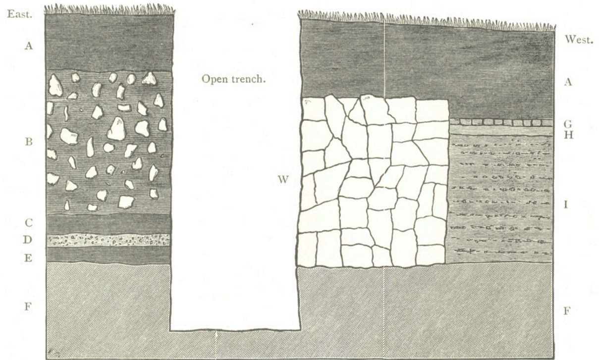
FIG. 8. —Section through the foundations of a buried Roman villa at Abinger. A A, vegetable mould ; B, dark earth full of stones, 13 inches in thickness ; C, black mould ; D, broken mortar ; E, black mould ; F F, undisturbed sub-soil ; G, tesserae ; H, concrete ; I, nature unknown ; W, buried wall.
