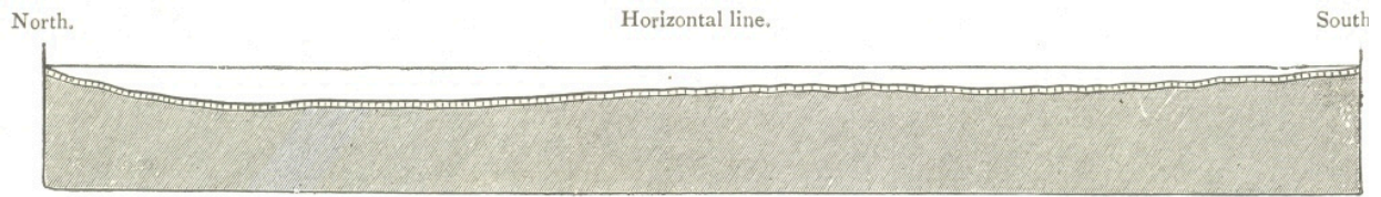
FIG. 13.—Section of the subsided floor of a room, paved with tesserae, at Silchester. Scale \frac{1}{4} inch.
