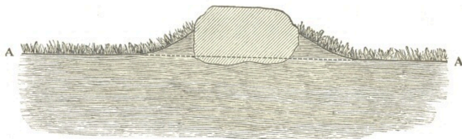
FIG. 6.—Transverse section across a large stone, which had lain on a grass-field for 35 years. A A, general level of the field. The underlying brick rubbish has not been represented. Scale \frac{1}{2} inch to one foot.
