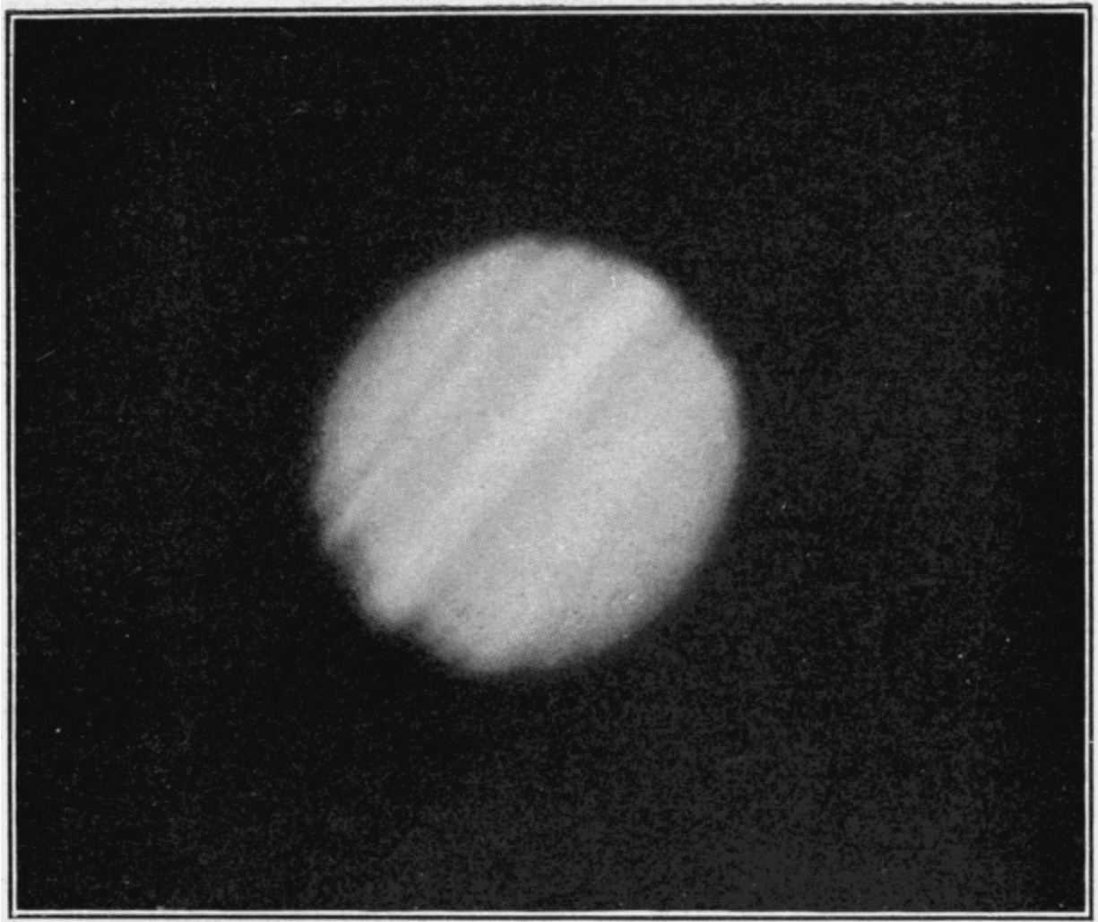
JUPITER, LARGEST OF THE PLANETS. The irregular belts change their mutual relation and shapes because they do not represent land, but are part of the atmosphere. ( Photo, Yerkes Observatory. )
