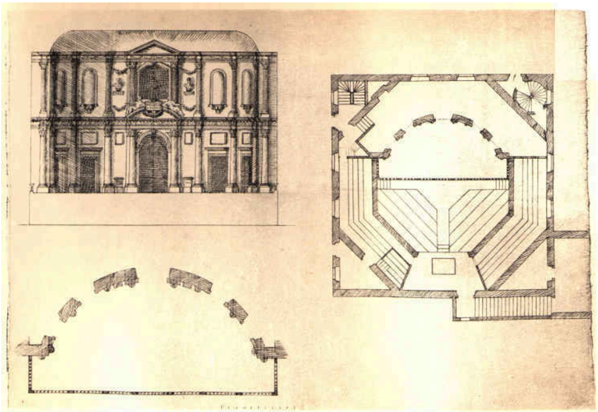
DESIGN BY INIGO JONES FOR THE COCKPIT THEATRE AT WHITEHALL NOW IN THE LIBRARY OF WORCESTER COLLEGE OXFORD
