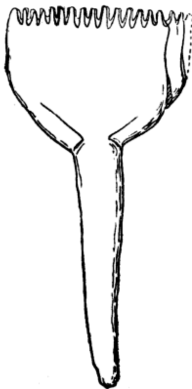
Fig. 22.—Weaver's Comb—a Beater-in. 19·5 cm. × 9·8 × 4·2 (7¾ in. × 3⅞ in. × 1⅝ in.) Gurob .
