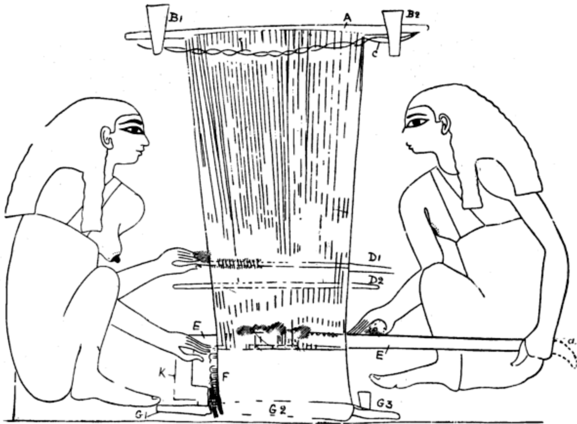
Fig. 6.—Horizontal Loom, Tomb of Chnem-hotep. Size of original: Height of the figures 9\frac{1}{4}" = 24.4 cm. Drawn by Mr. N. de G. Davies, and now published for the first time by permission of Mr. F. Ll. Griffith.
