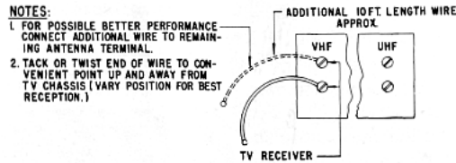
FIG. 9—ANTENNA CONNECTIONS AT CABINET BACK
