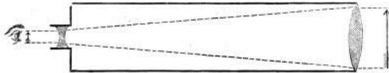
The Galilean Telescope.
