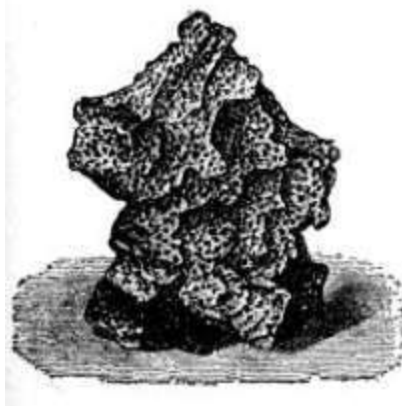
Meteorite found in Chili in 1866.
