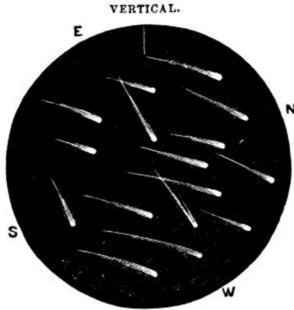
Flight of Telescopic Meteors seen by W. R. Brooks, Nov. 28, 1883.
