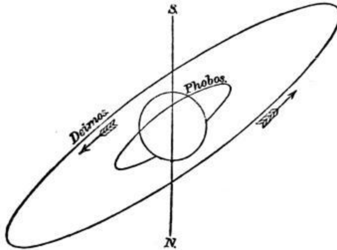
Orbits of the Satellites of Mars.
