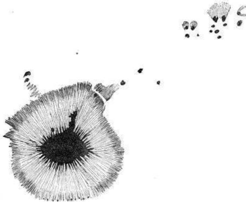
Sun-spot of June 19, 1889, 2 h P.M.
