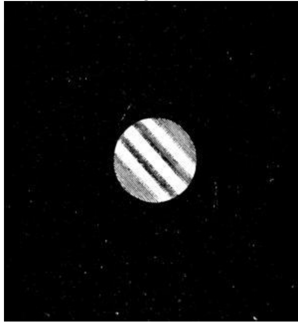
Uranus and his Belts. 1884.
