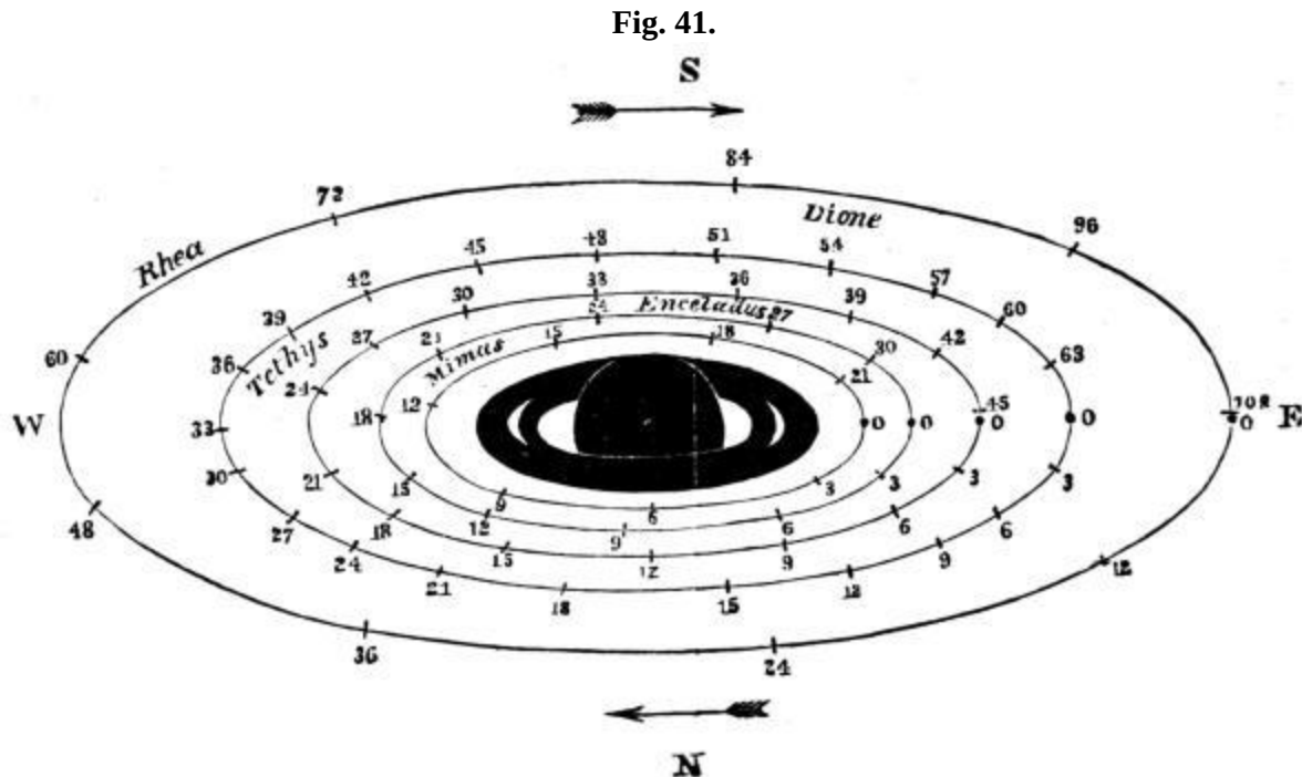
Apparent Orbits of the Five Inner Satellites of Saturn, as seen in an Inverting Telescope.
