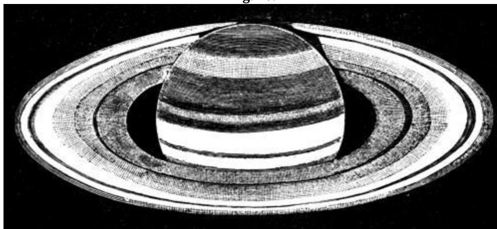
Saturn, as observed by F. Terby, February 1887.
