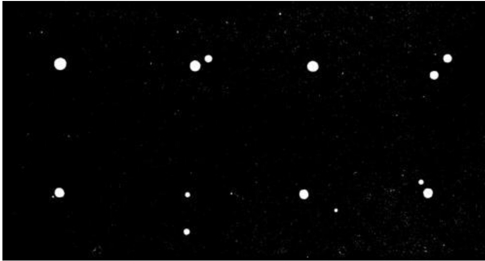
Double Stars.
