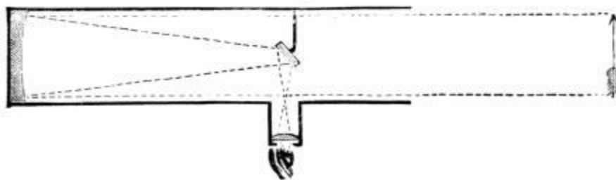
Newtonian Telescope.
