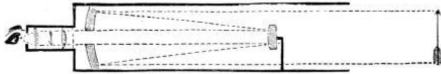
Cassegrainian Telescope.
