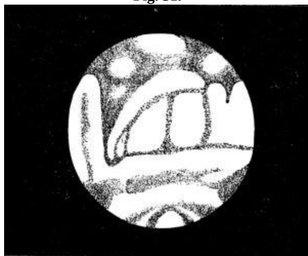
Mars, 1836, April 13, 9 h 50 m ; long. 332°. (10-inch reflector; power 252.)
