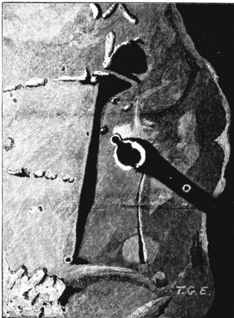
Birt, Birt A, and the Straight Wall. 1883, Feb. 15, 6 h to 8 h 40 m . (T. Gwyn Elger.)
