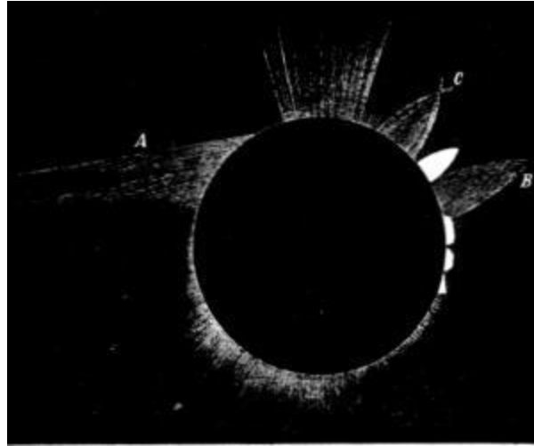
Total Solar Eclipse of August 19, 1887.
