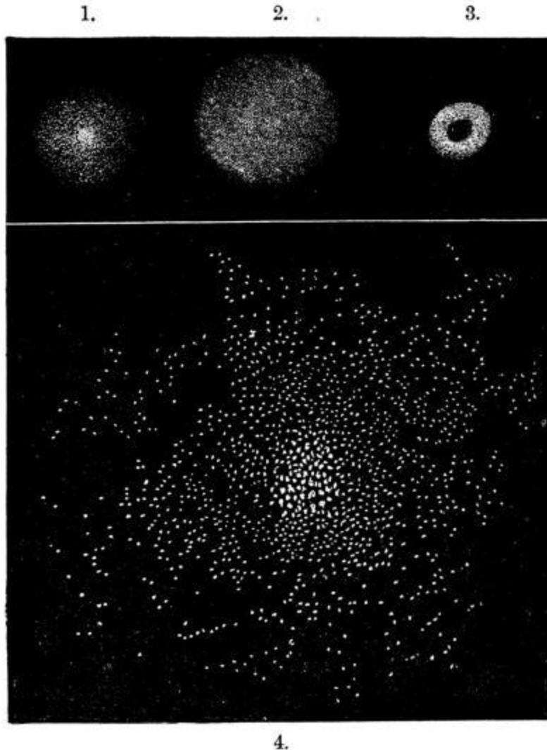
1. Nebula with bright centre. 2. Planetary Nebula. 3. Ring-nebula in Lyra. 4. Star-cluster in Hercules.
