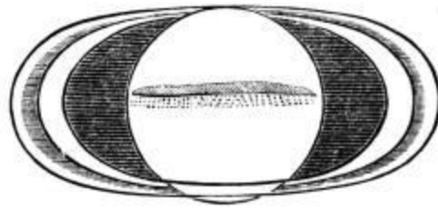
Saturn, as observed by Cassini in August 1676.
