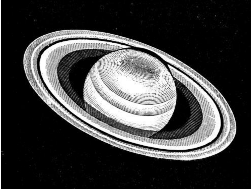
Saturn, 1885, Dec. 23, 7 h 54 m . (10-inch reflector, power 252.)
