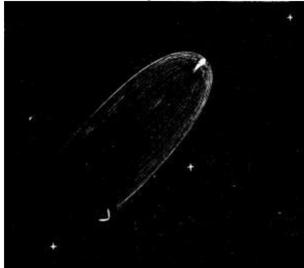
Comet 1862 III. (Aug. 19, 1862).
