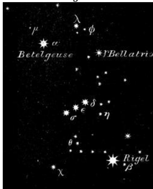
The constellation Orion.
