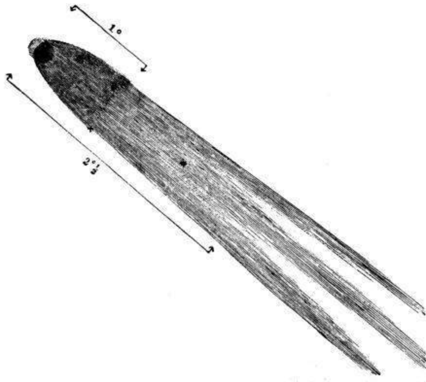
Pons's Comet (1812). Telescopic view. 1884, January 21, 13 h 18 m . (5-inch refractor; comet-eyepiece, field 1-1/4°. E. E. Barnard.)
