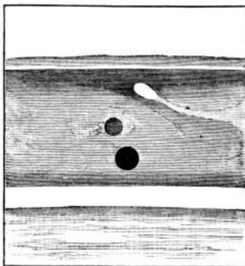
Shadows of Jupiter's Satellites II. and III. near an equatorial white spot (Jan. 1, 1885, 7 h 20 m A.M.).
