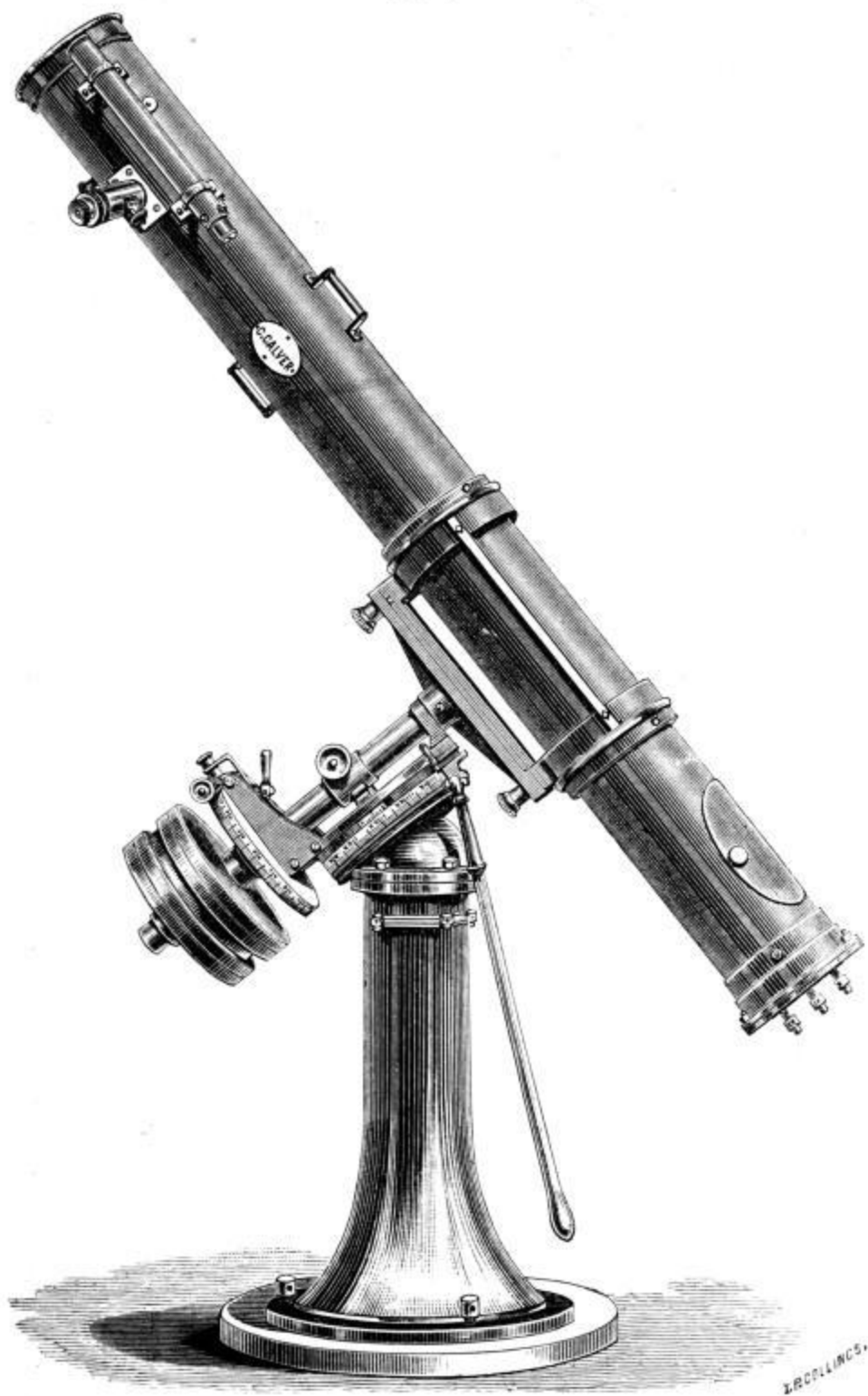
10-inch Reflecting-Telescope on a German Equatoreal, by Calver.
