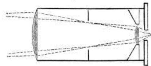
Huygens's negative eyepiece.
