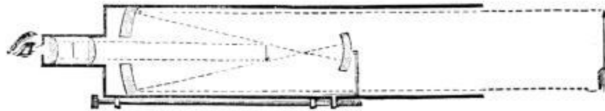
Gregorian Telescope.
