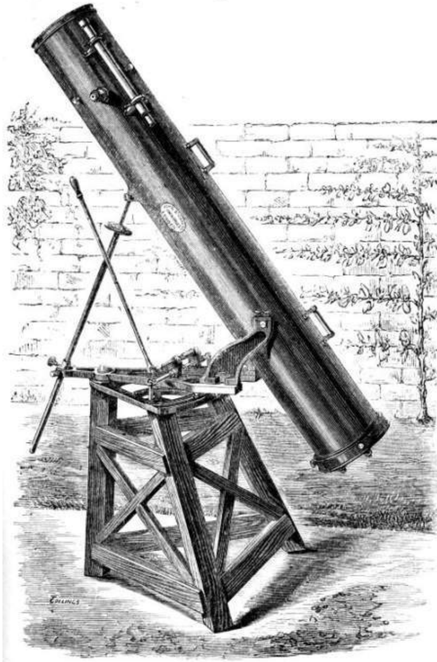
The Author's Telescope: a 10-inch With-Browning Reflector.
