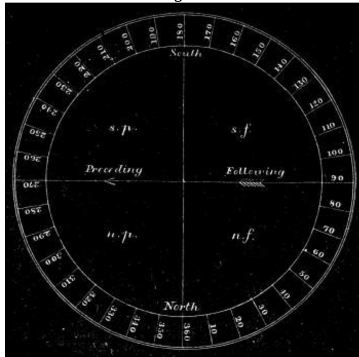
Diagram illustrating the Measurement of Angles of Position.
