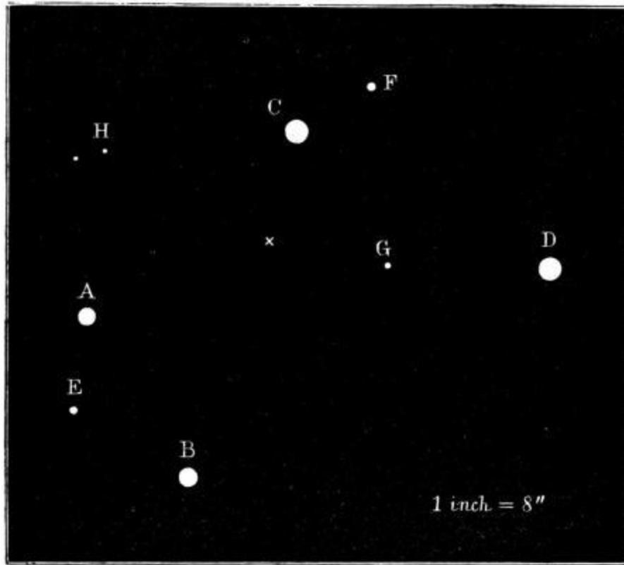
The Trapezium in Orion, as seen with the 36-inch refractor.
