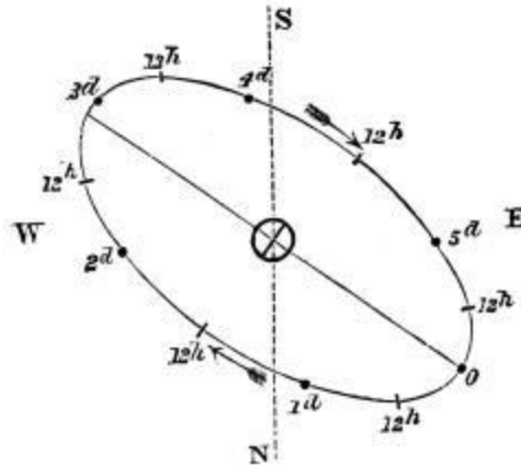
Apparent Orbit of the Satellite of Neptune, as seen in an Inverting Telescope.
