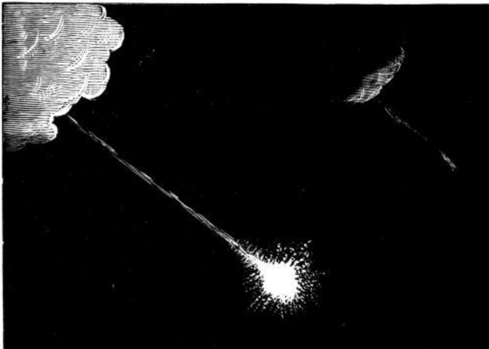
Fireball of Nov. 23, 1877, 8 h 24 m , emerging from behind a cloud. (Drawn by J. Plant, Salford.)
