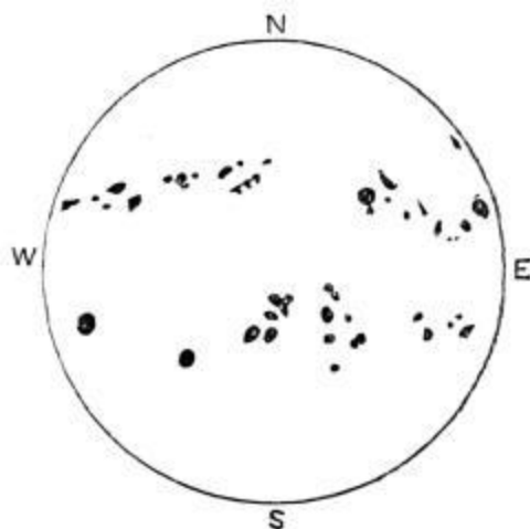
Belts of Sun-spots, visible October 29, 1868.
