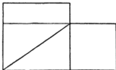
Addition zweier Quadrate.
