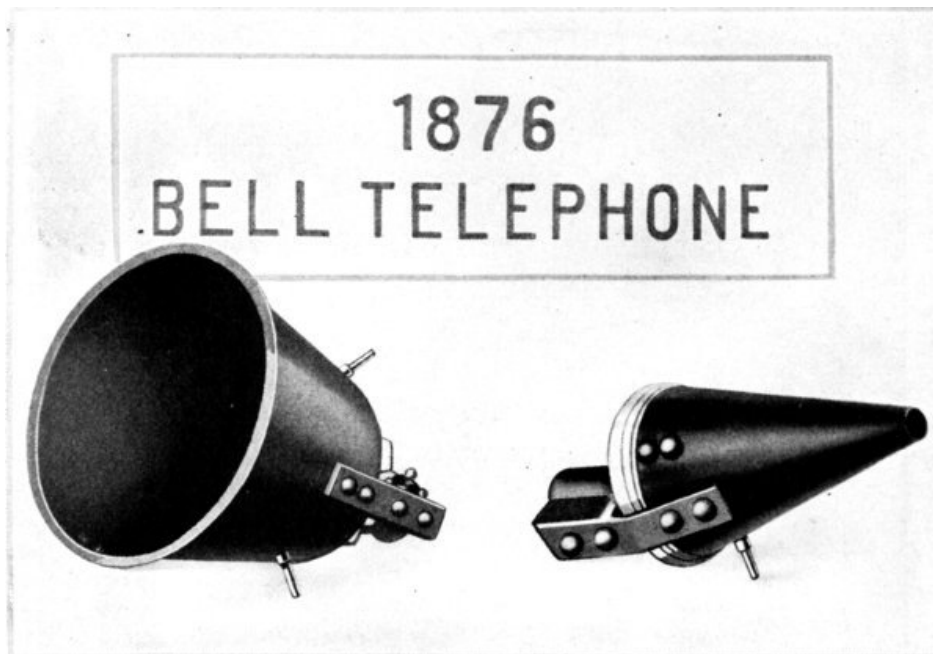
1876 BELL TELEPHONE
