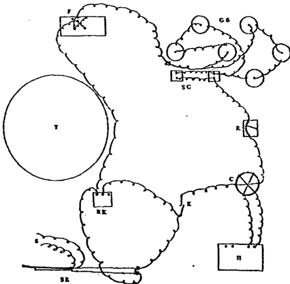
FIG. 6. General Plan of Apparatus in Diagram. H , Hipp Chronoscope; R , rheostat; C , commutator; SC , storage cells; GB , 'Excello' gravity battery; F , Cattell's falling screen; T , reaction table; RK , reaction key; SK , Stimulating apparatus; K , key in chronoscope circuit; S , stimulus circuit.
