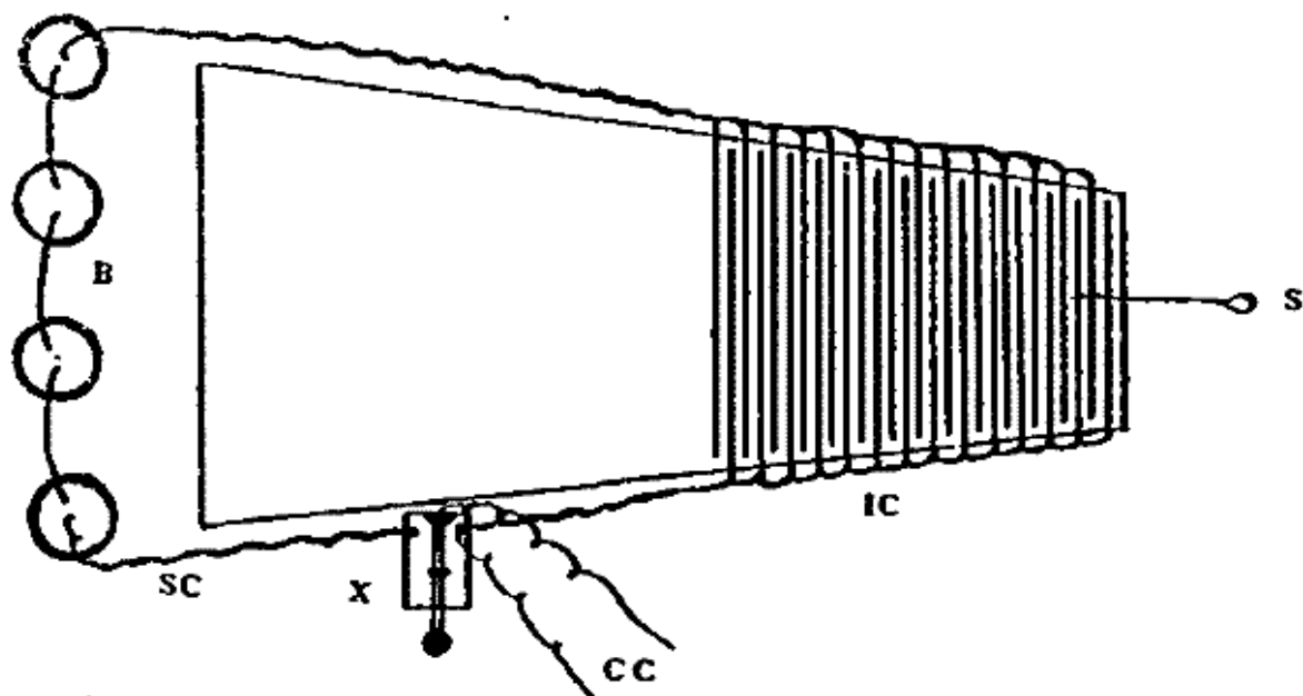
FIG. 9. Ground Plan of Reaction Box for Electrical Stimuli (Group 2). IC, interrupted circuits; CC, chronoscope circuit; X, key for making stimulus circuit and breaking chronoscope circuit; B, stimulus battery; S, string from reaction key to animal. Scale 1/2.
