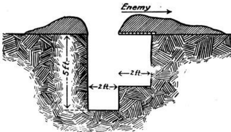
PLATE 19a.—Overhead cover.
