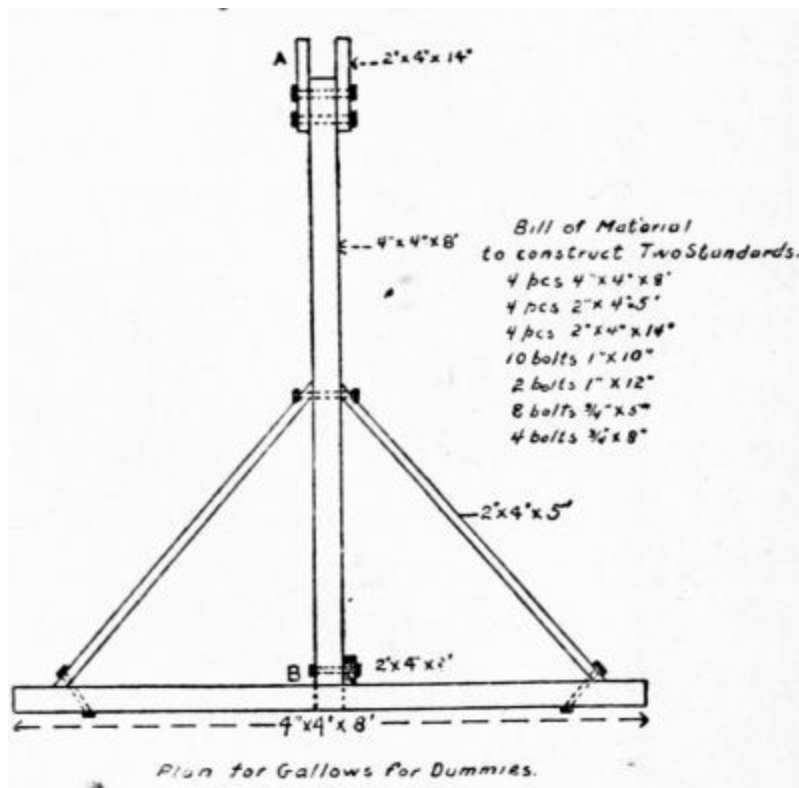
Plan for Gallows for Dummies.
