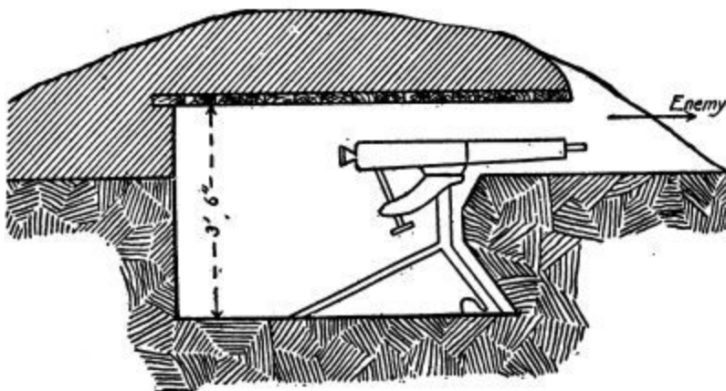
PLATE 26.—Profile of type of cover for machine gun.
