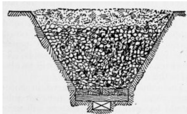
PLATE 9.—Vertical fougass.
