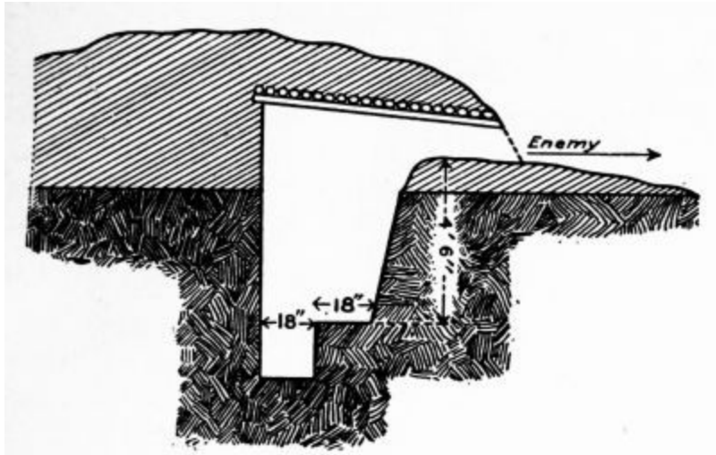
PLATE 19.—Overhead cover.
