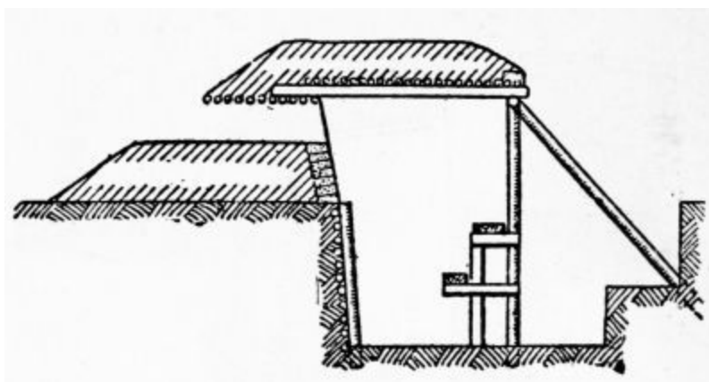
PLATE 20.—Overhead cover.
