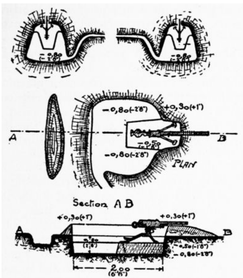
PLATE 27.—Type of cover for machine guns.
