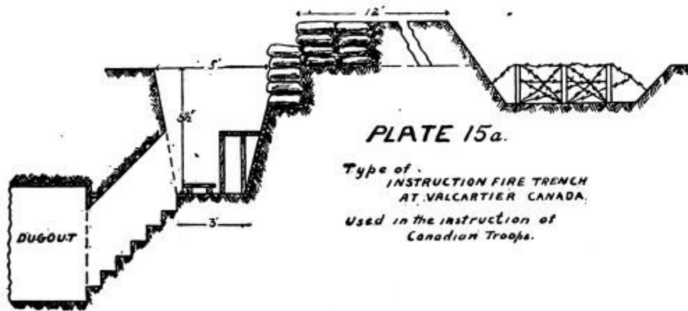
PLATE 15a. Type of INSTRUCTION FIRE TRENCH AT VALCARTIER CANADA.
