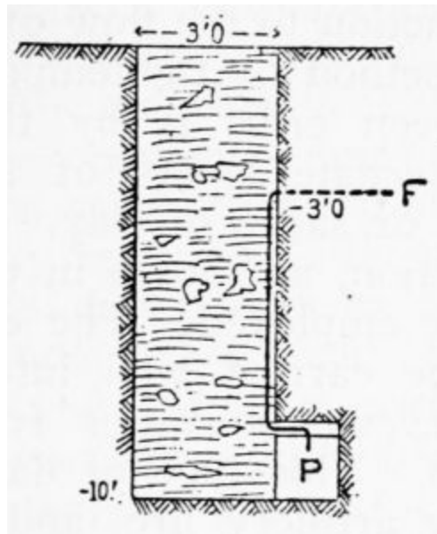
n: PLATE 9a.—Land mine. F , Line from powder charge to battery. P , Powder charge.
