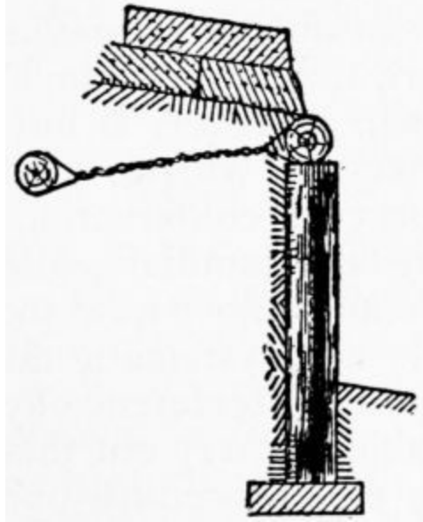
PLATE 38.—Timber revetment.
