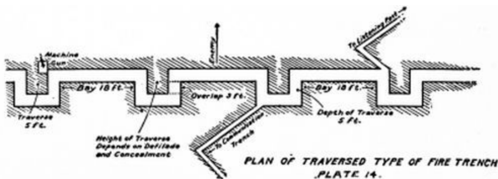
PLAN OF TRAVERSED TYPE OF FIRE TRENCH PLATE 14.
