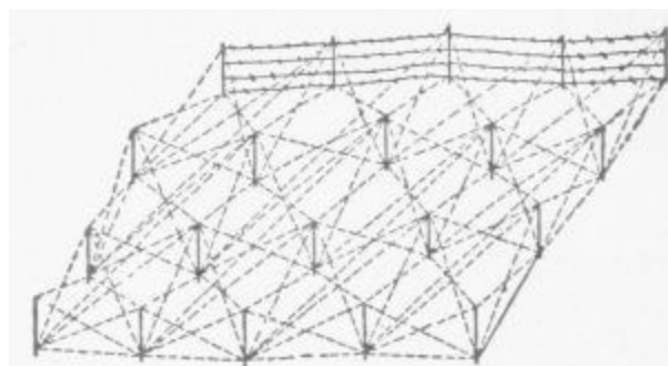
PLATE 4a.—Plan of wire entanglement.
