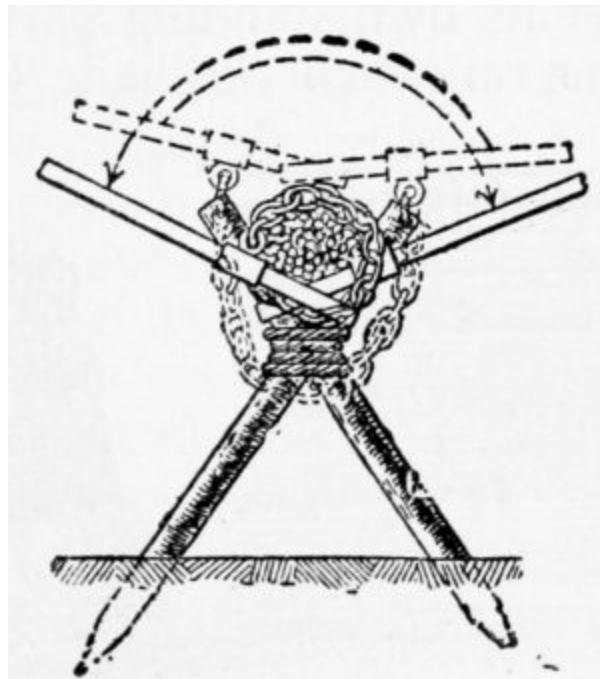
PLATE 30.—Method of using the fascine choker.
