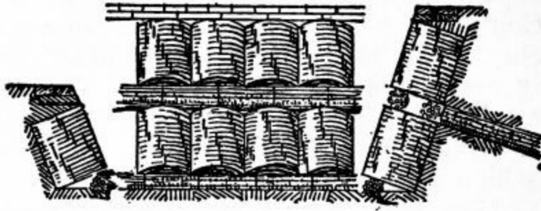
PLATE 37.—Methods of use of gabion.
