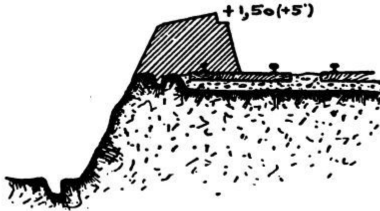
PLATE 27u.—Arrangement of a railroad embankment.
