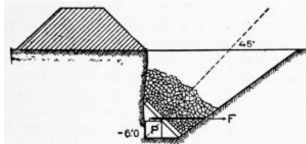
PLATE 8.—Fougass.
