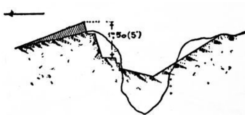
PLATE 27p.—Arrangement of a large ditch.
