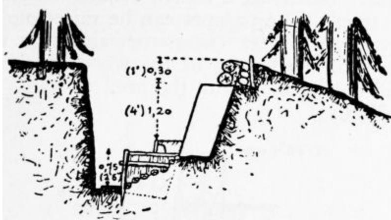
PLATE 27w.—Arrangement of a hedge.
