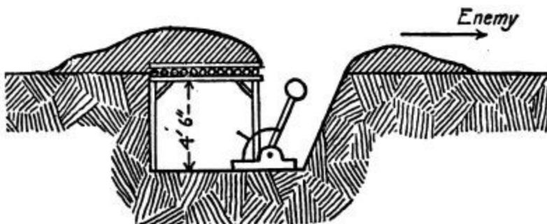
PLATE 25.—Profile of trench mortar emplacement.
