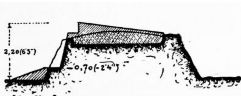
PLATE 27t.—Road embankment, defended from the rear.
