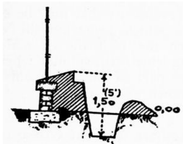
PLATE 28a.—Arrangement of an iron fence built on a low wall.
