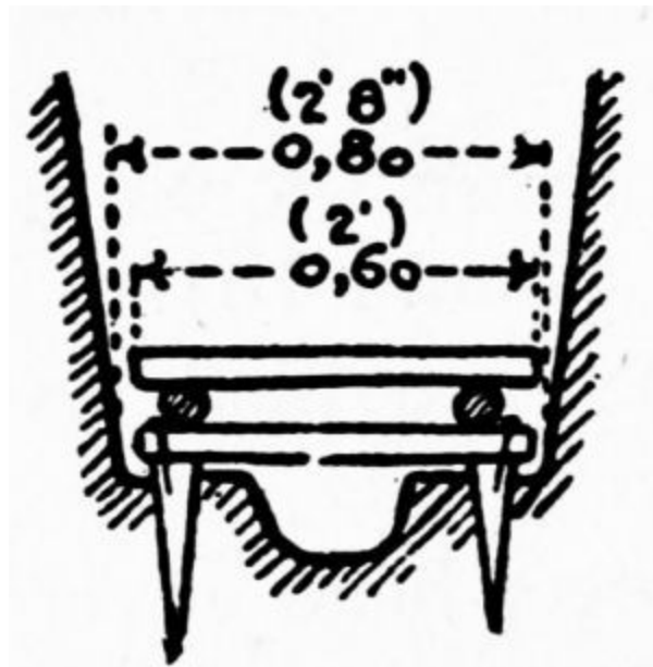
PLATE 17.—Details of trench drainage.
