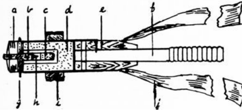
PLATE 41b.—British hand grenade No. 1.
