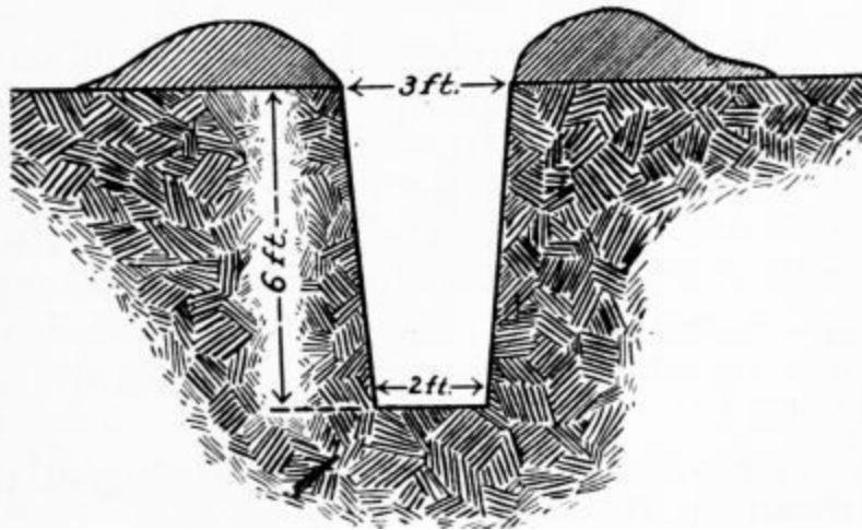
PLATE 23.—Type of communication trench.
