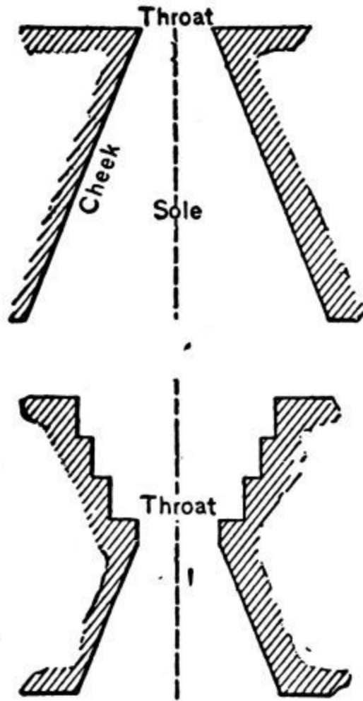
PLATE 21.—Types of loopholes.
