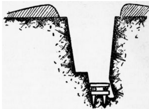
PLATE 16.—Method of draining trench.
