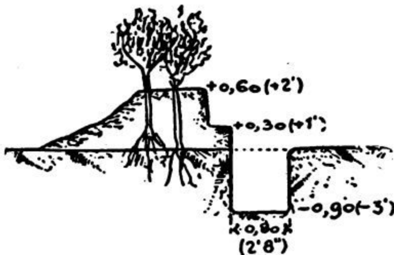
PLATE 27v.—Arrangement of a sunken road.
