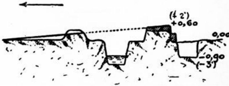
PLATE 27q.—Arrangement of a ditch full of water.
