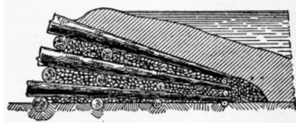
PLATE 10.—Dam construction.
