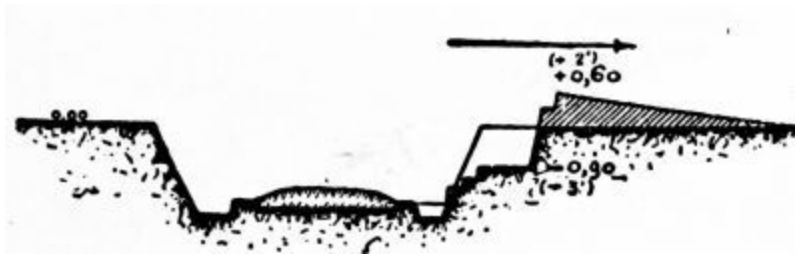
PLATE 27n.—Arrangement for a sunken road defended on the side towards the enemy.
