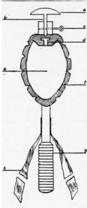
PLATE 41C.—The latest type British hand grenade.
