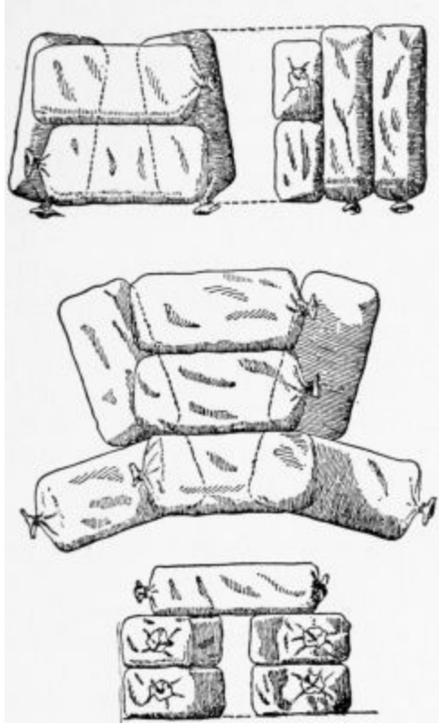
PLATE 22.—Methods of constructing loopholes with sandbags.
