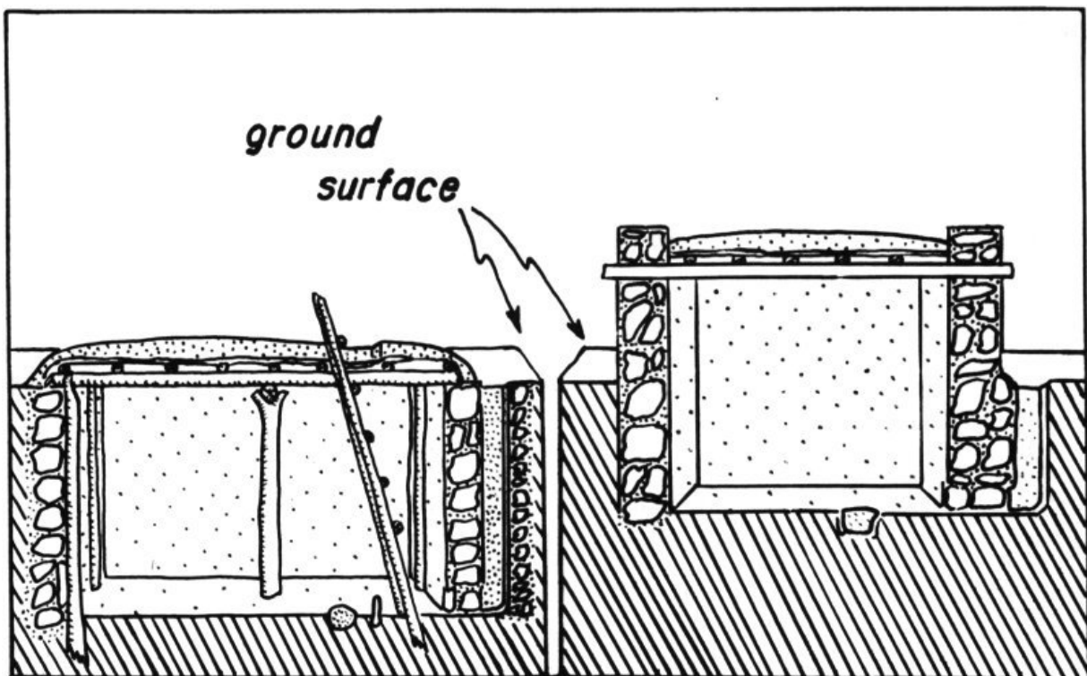
Reconstruction of two types of pithouses found in this region. Note the two methods of roofing and the ventilator at right.
