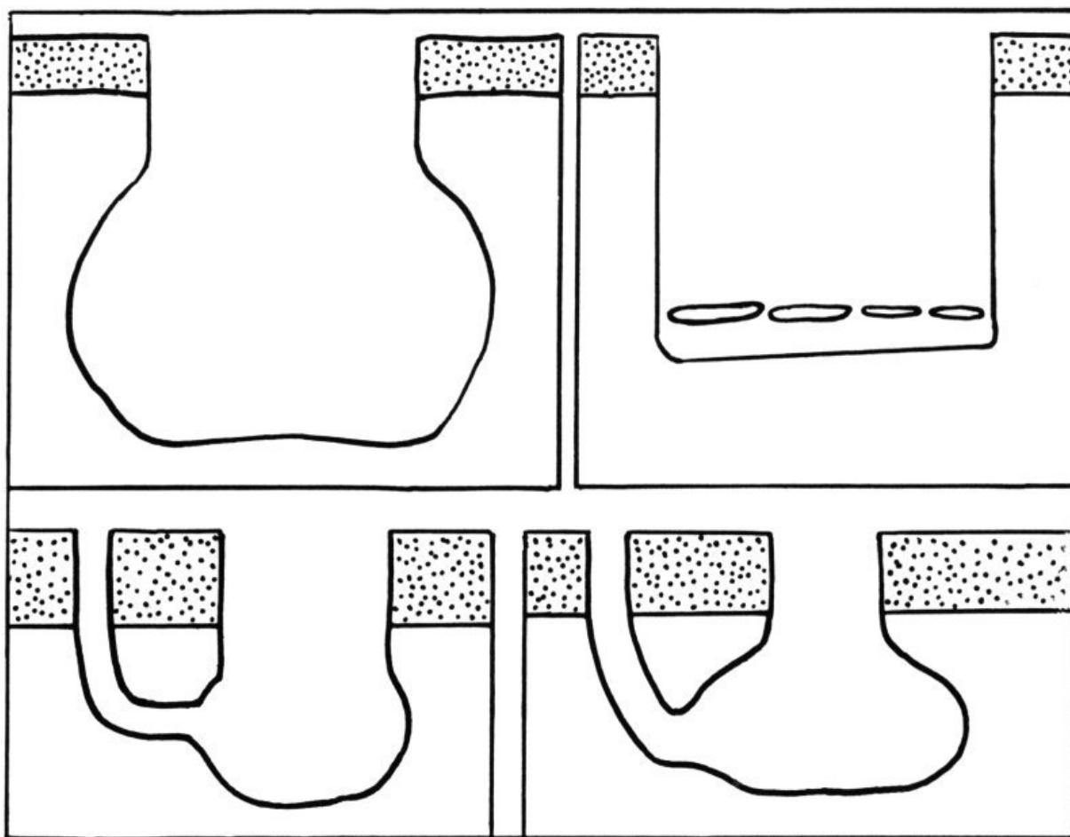
Cross-sections of various pits near Nalakihi.
