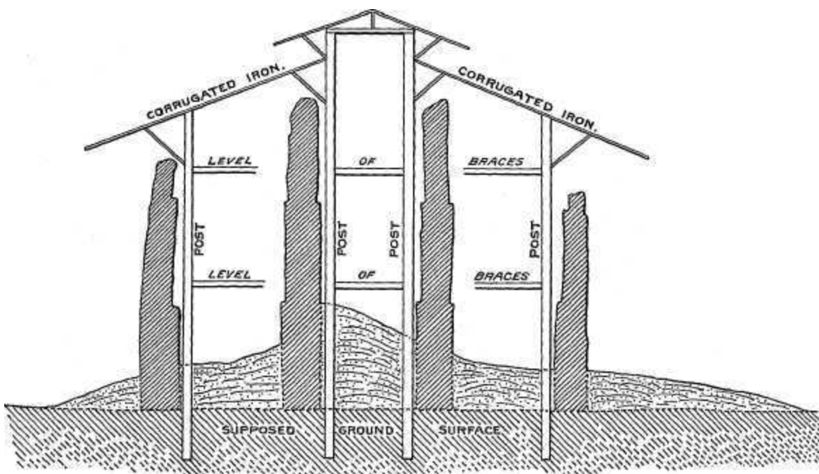
SECTION THROUGH A-B OF ROOF PLAN. SHOWING SUGGESTED ROOF SUPPORT
