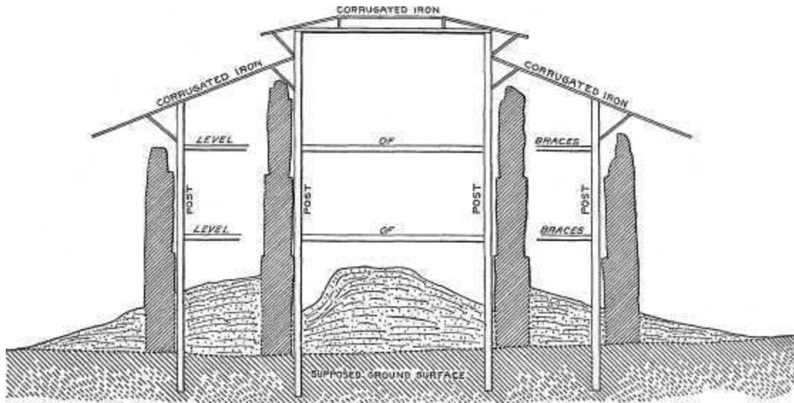
SECTION THROUGH C-D OF ROOF PLAN, SHOWING SUGGESTED ROOF SUPPORT
