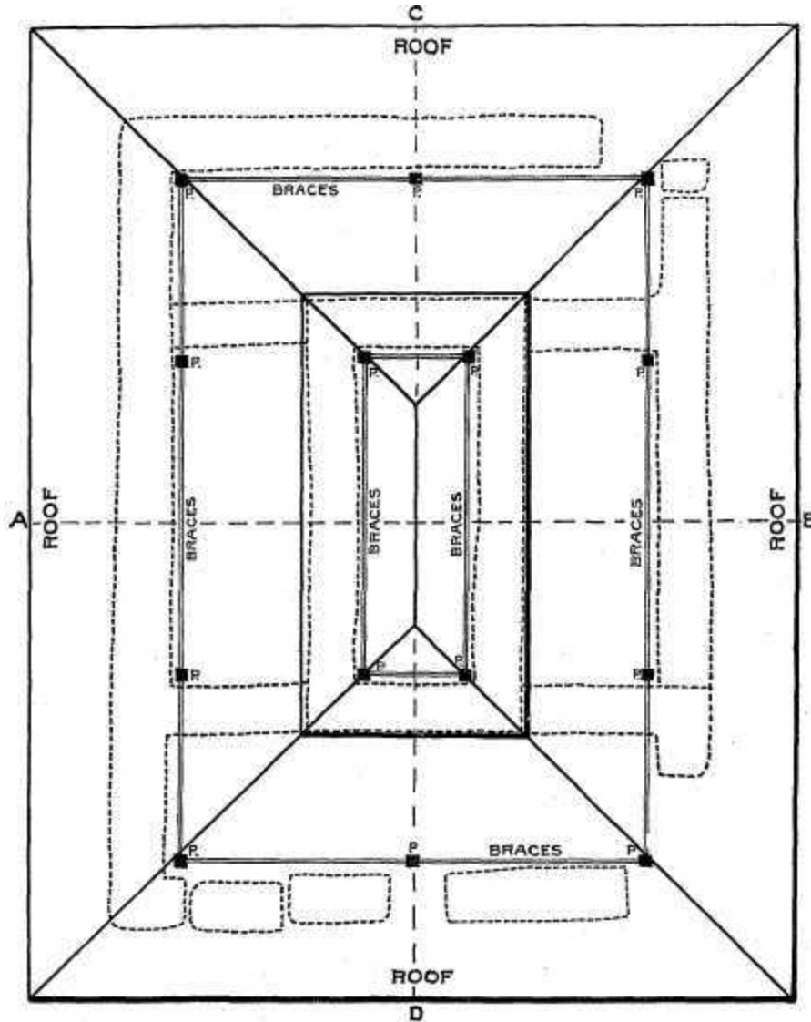
SUGGESTED PLAN OF ROOF AND SUPPORT
