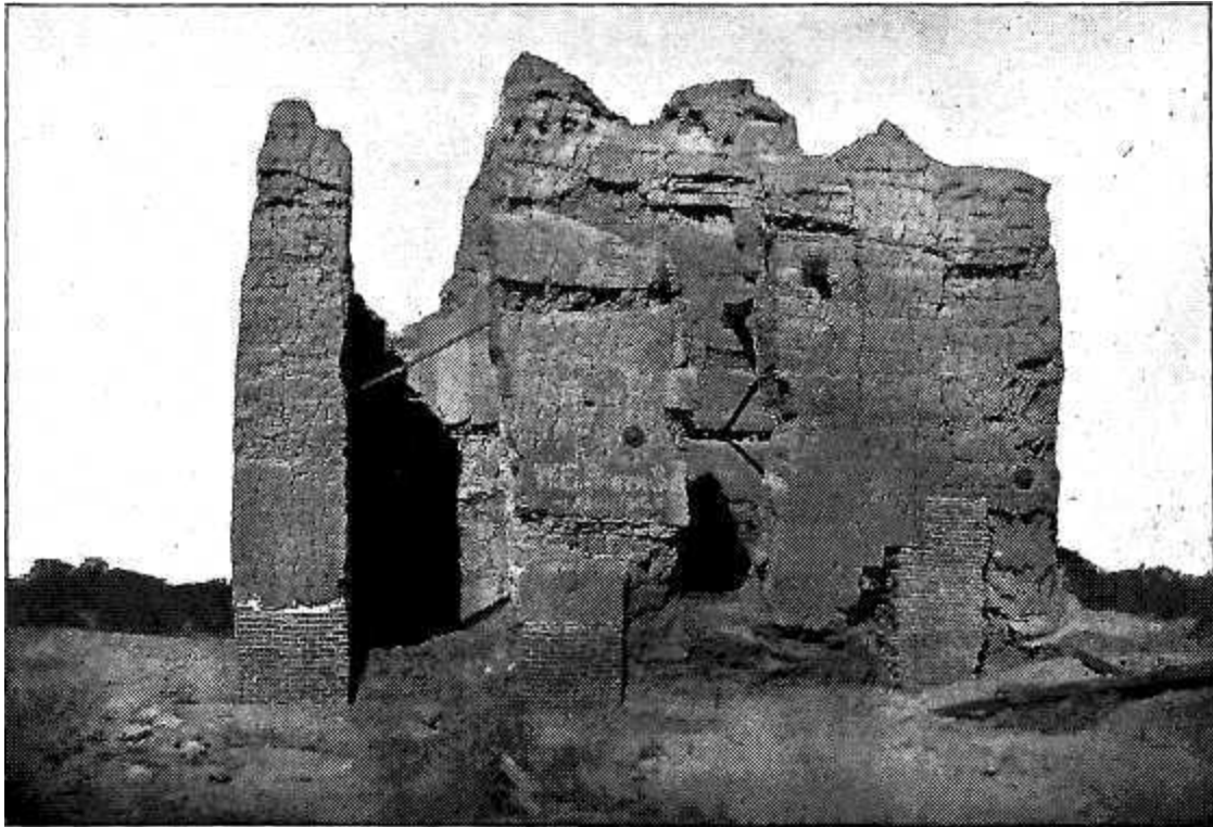
SOUTH FRONT OF THE RUIN, SHOWING UNDERPINNING AND ENDS OF TIE-RODS
