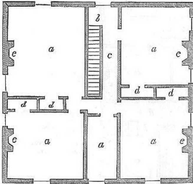
Fig. 30. Second Story.
