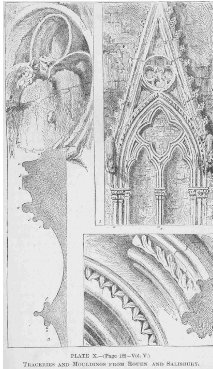
PLATE X.—(Page 122—Vol. V.) TRACERIES AND MOULDINGS FROM ROUEN AND SALISBURY.
